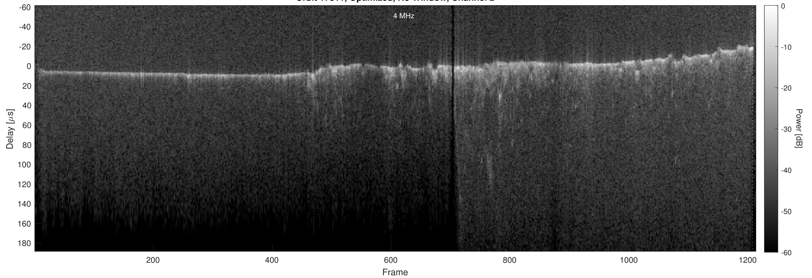
Orbit 17811, Optimized, No Window, Channel 2
