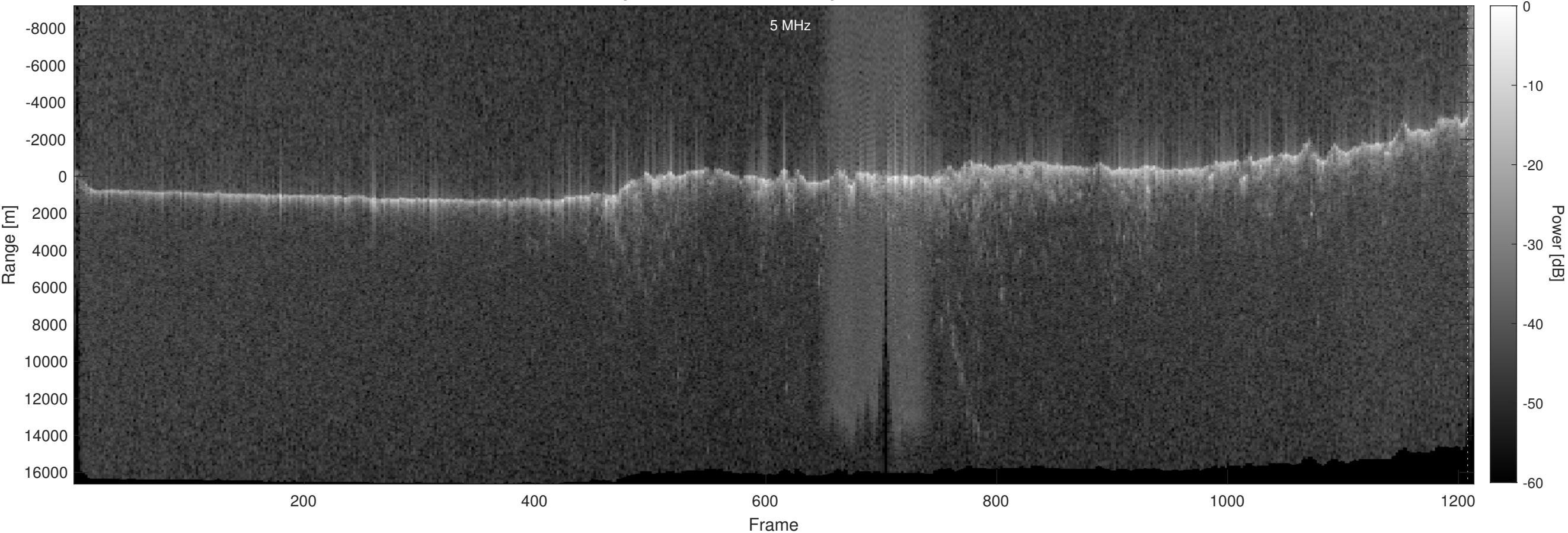
Orbit 17811, Optimized, No Window, Depth-Corrected, Channel 2
