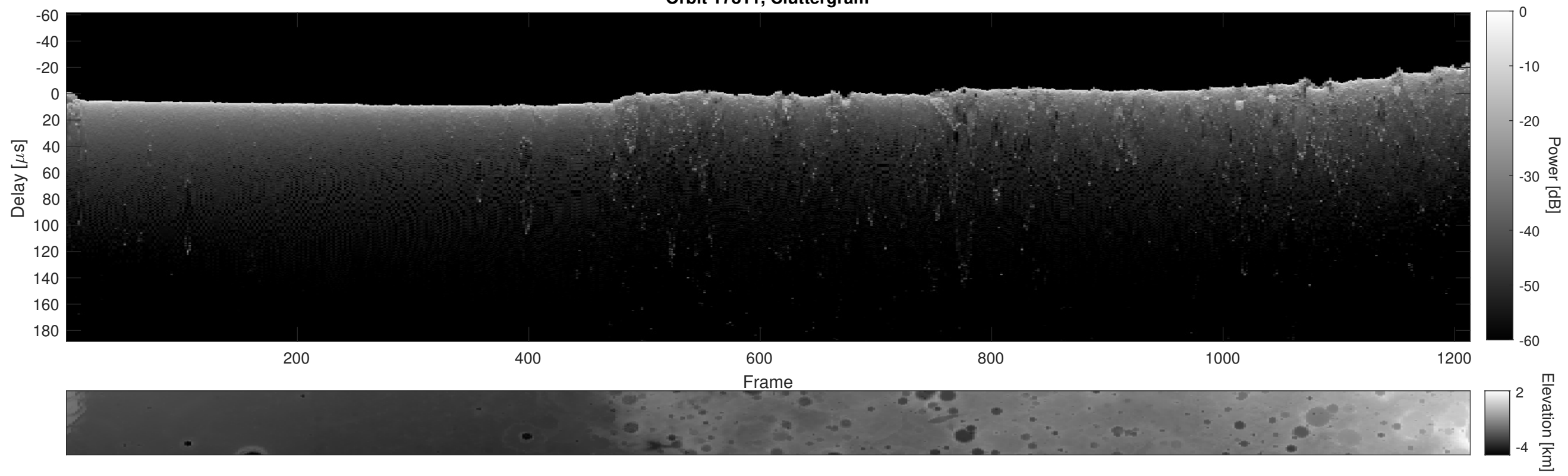
Orbit 17811, Cluttergram
