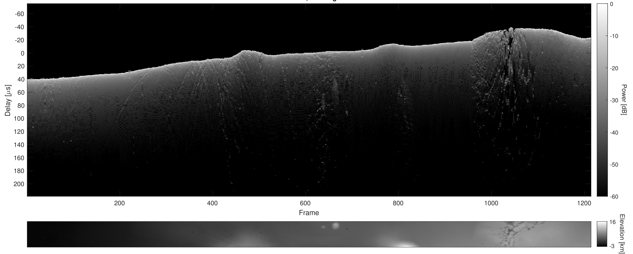
Orbit 17812, Cluttergram
