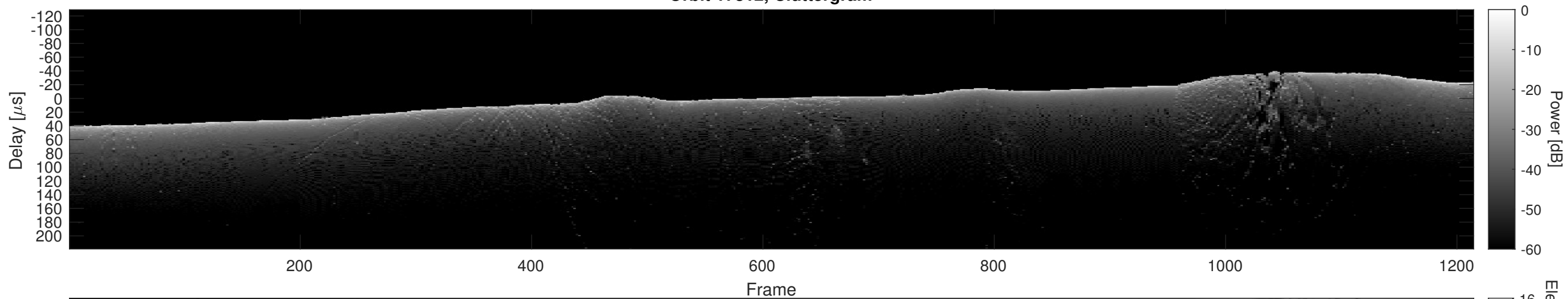
Orbit 17812, Cluttergram
