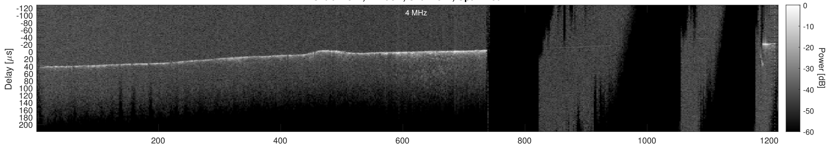
Orbit 17812, Cluttergram
