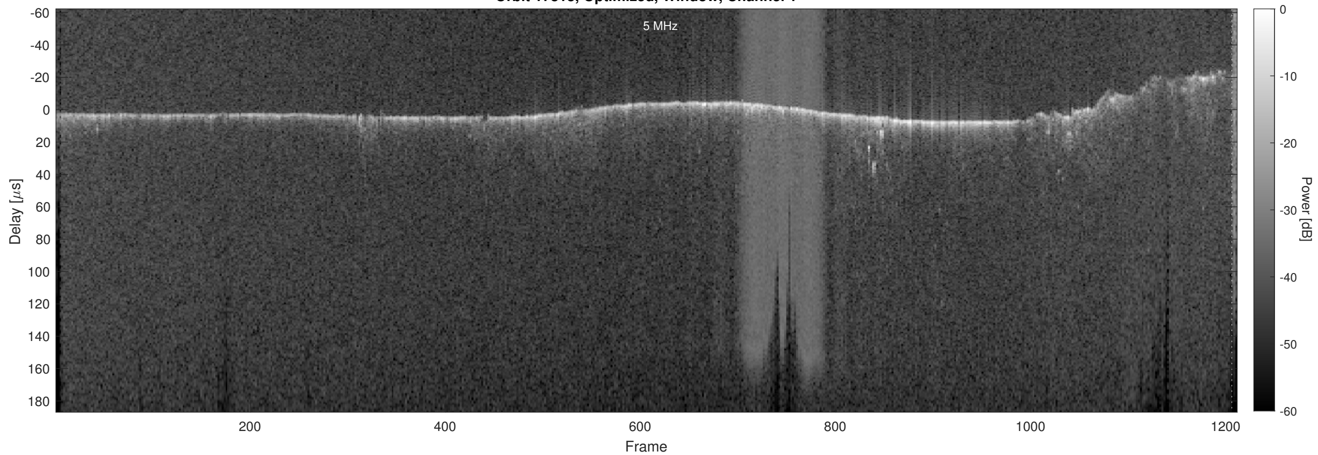
Orbit 17813, Optimized, Window, Channel 2
