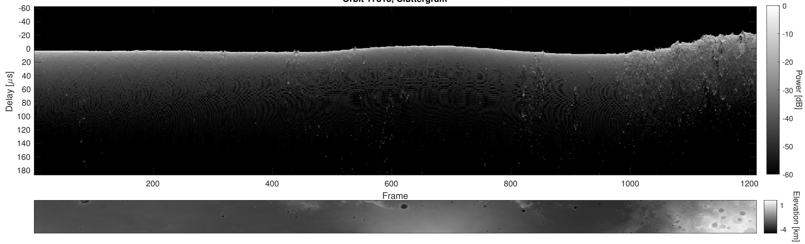
Orbit 17813, Cluttergram
