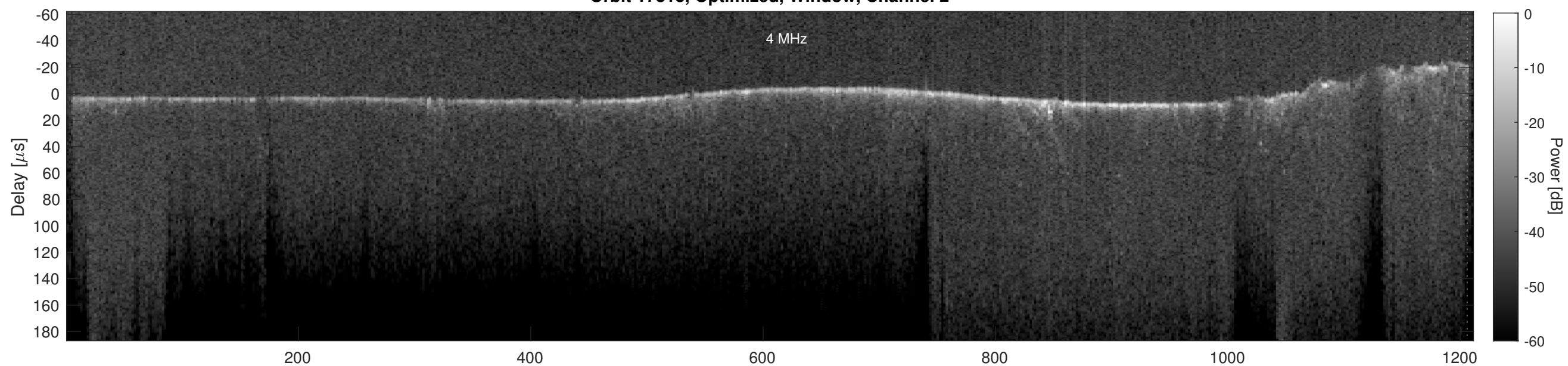
Orbit 17813, Cluttergram
