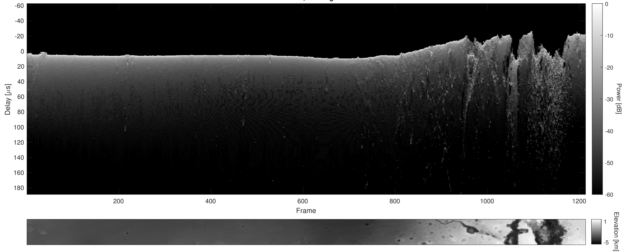
Orbit 17815, Cluttergram
