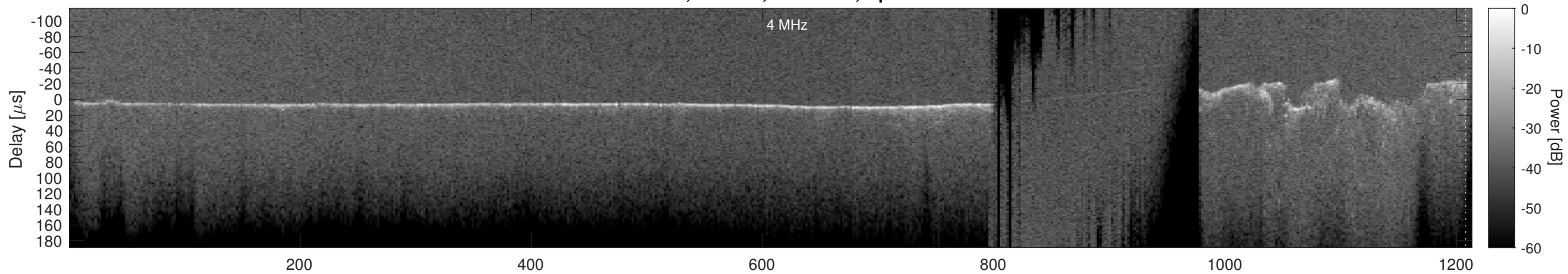
Orbit 17815, Cluttergram
