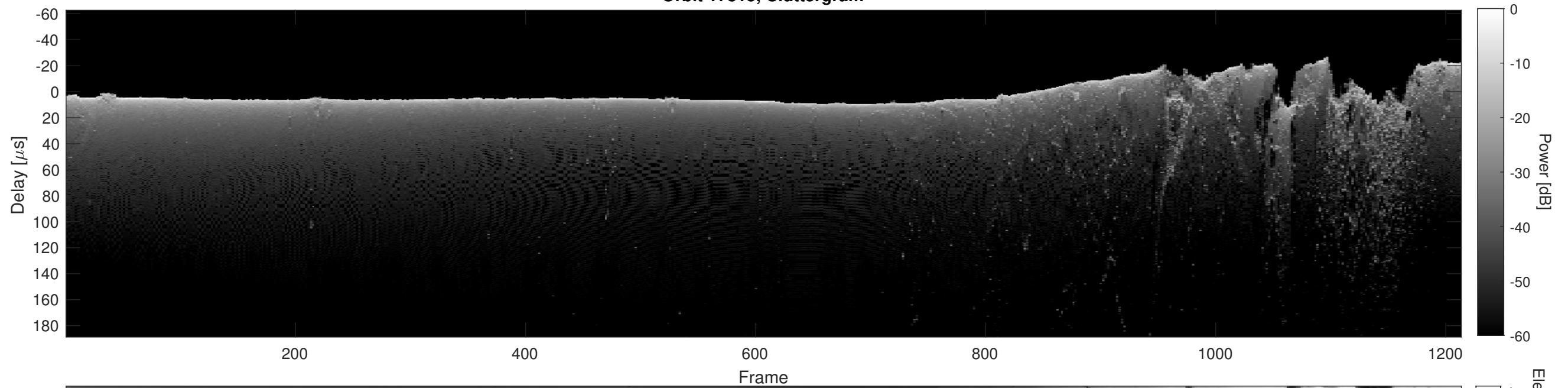
Orbit 17815, Cluttergram
