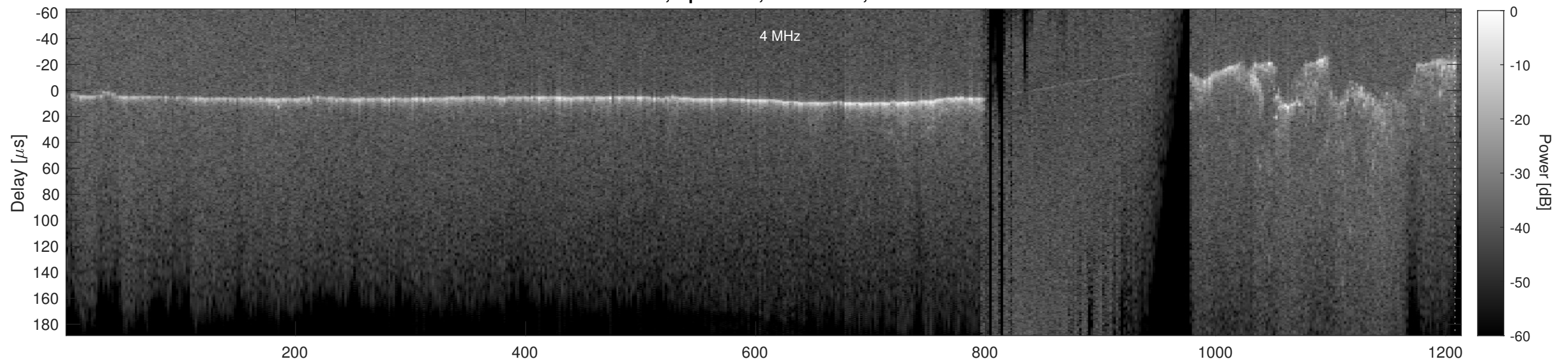
Orbit 17815, Cluttergram
