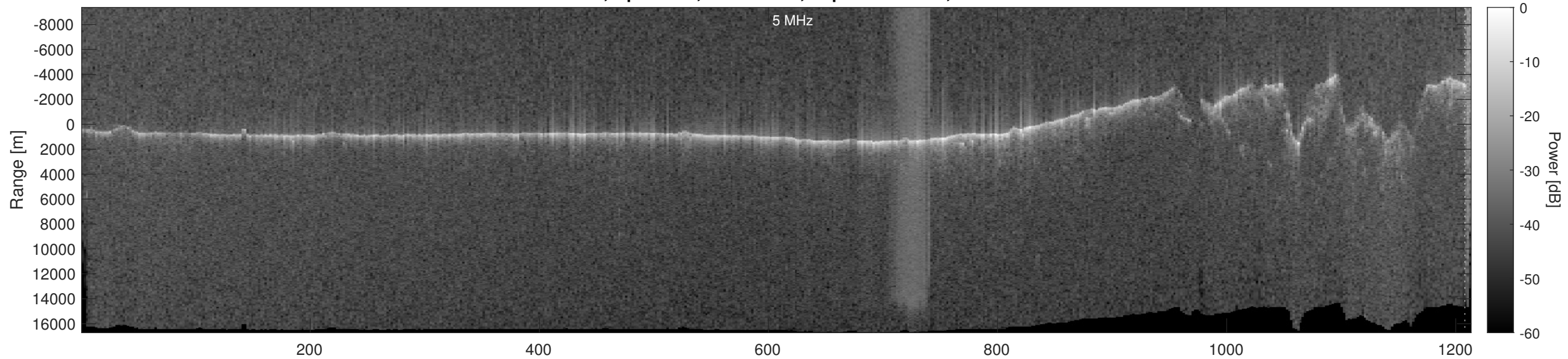
Orbit 17815, Optimized, No Window, Depth-Corrected, Channel 2
