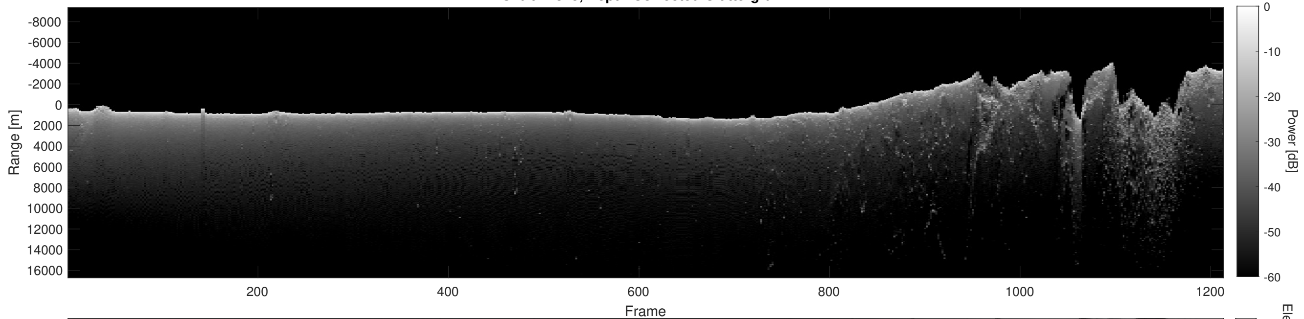
Orbit 17815, Depth-Corrected Cluttergram
