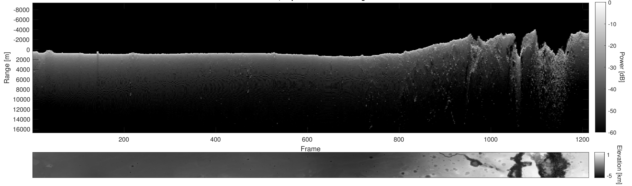
Orbit 17815, Depth-Corrected Cluttergram
