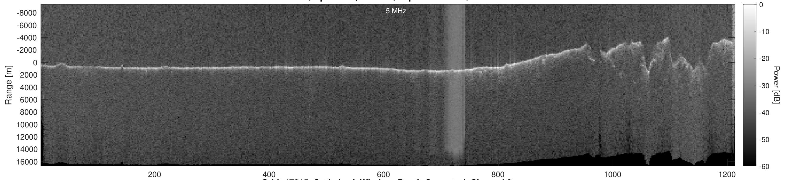
Orbit 17815, Optimized, Window, Depth-Corrected, Channel 2
