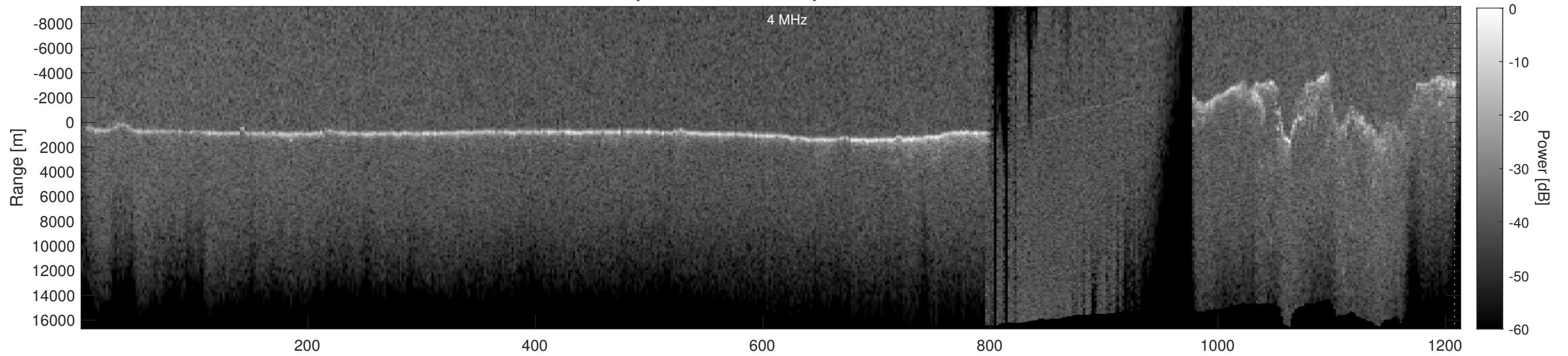
Orbit 17815, Depth-Corrected Cluttergram
