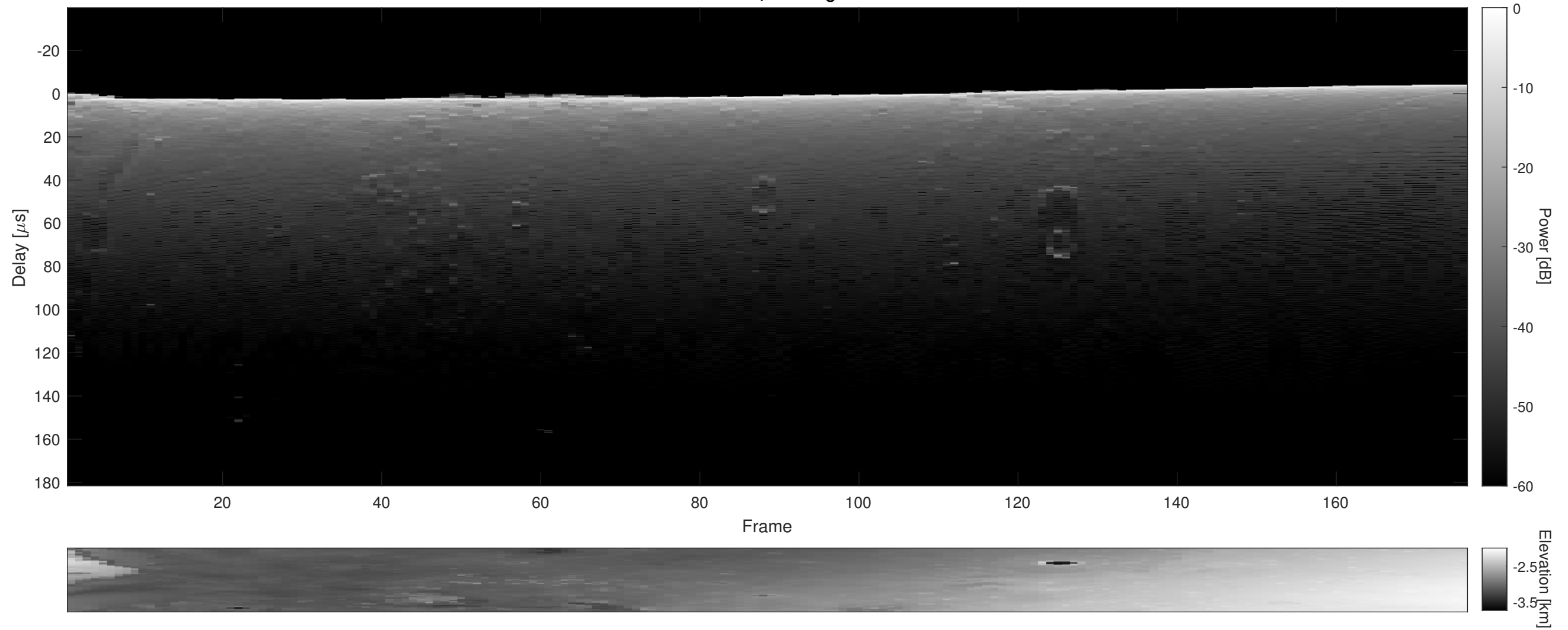
Orbit 17819, Cluttergram
