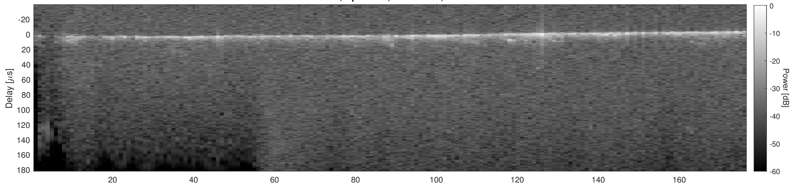
Orbit 17819, Cluttergram
