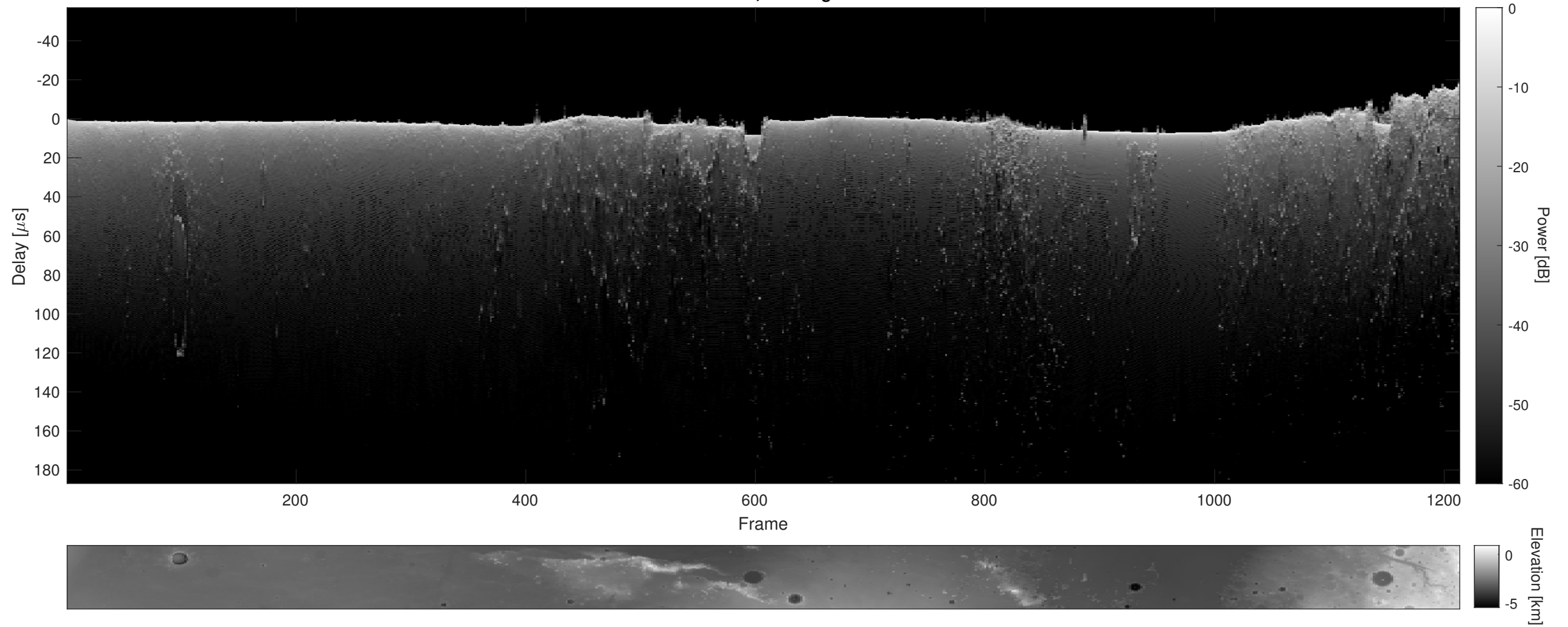
Orbit 17820, Cluttergram
