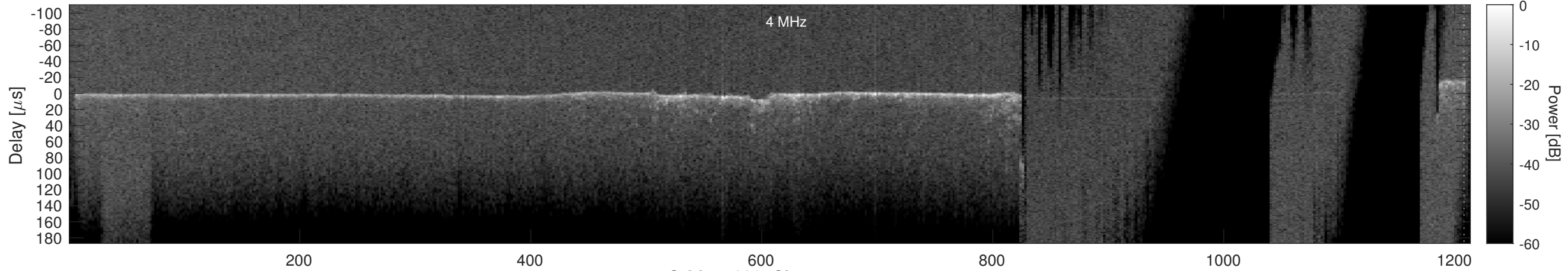
Orbit 17820, Cluttergram
