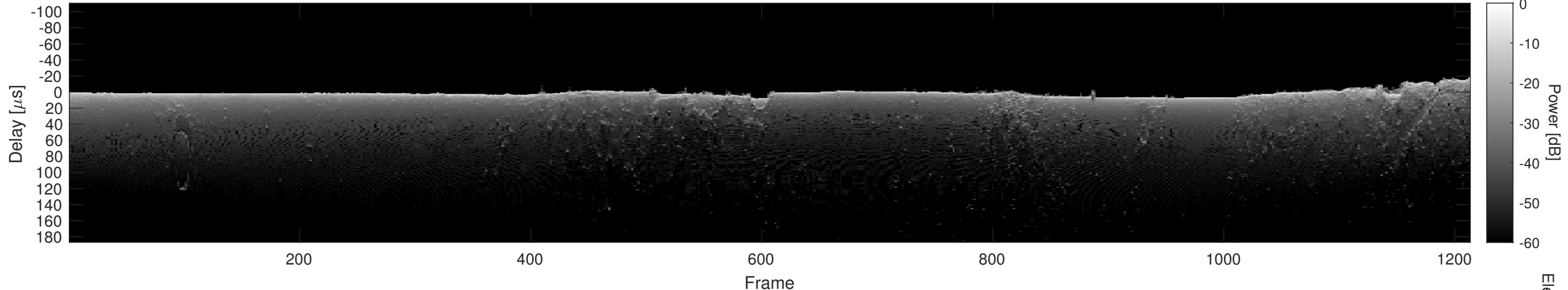
Orbit 17820, Cluttergram
