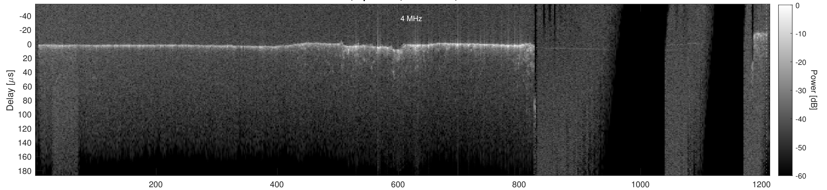
Orbit 17820, Cluttergram
