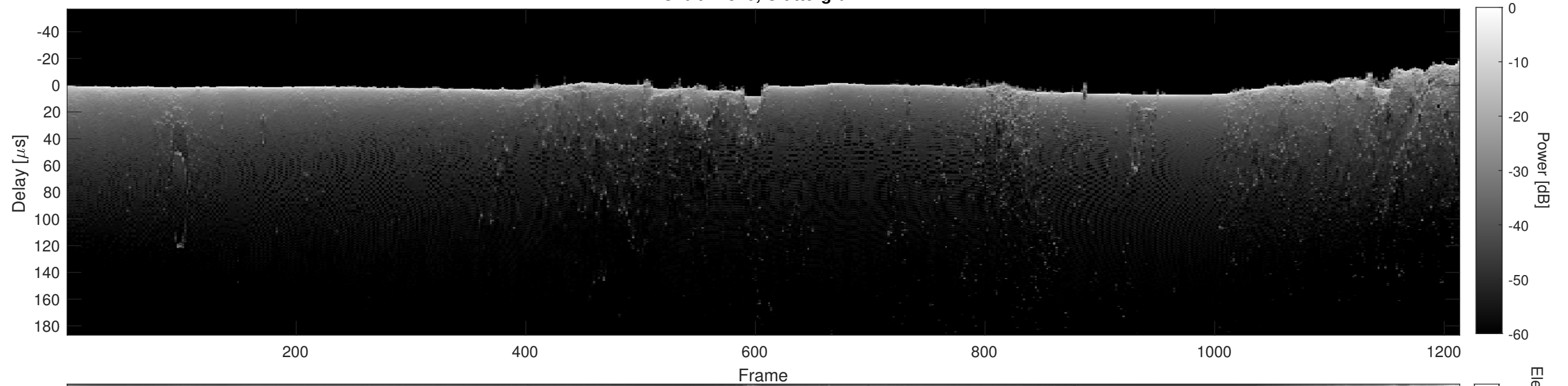
Orbit 17820, Cluttergram
