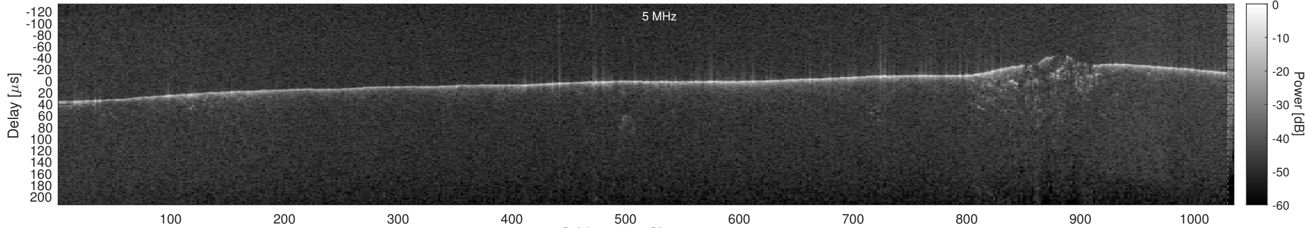
Orbit 17821, Cluttergram
