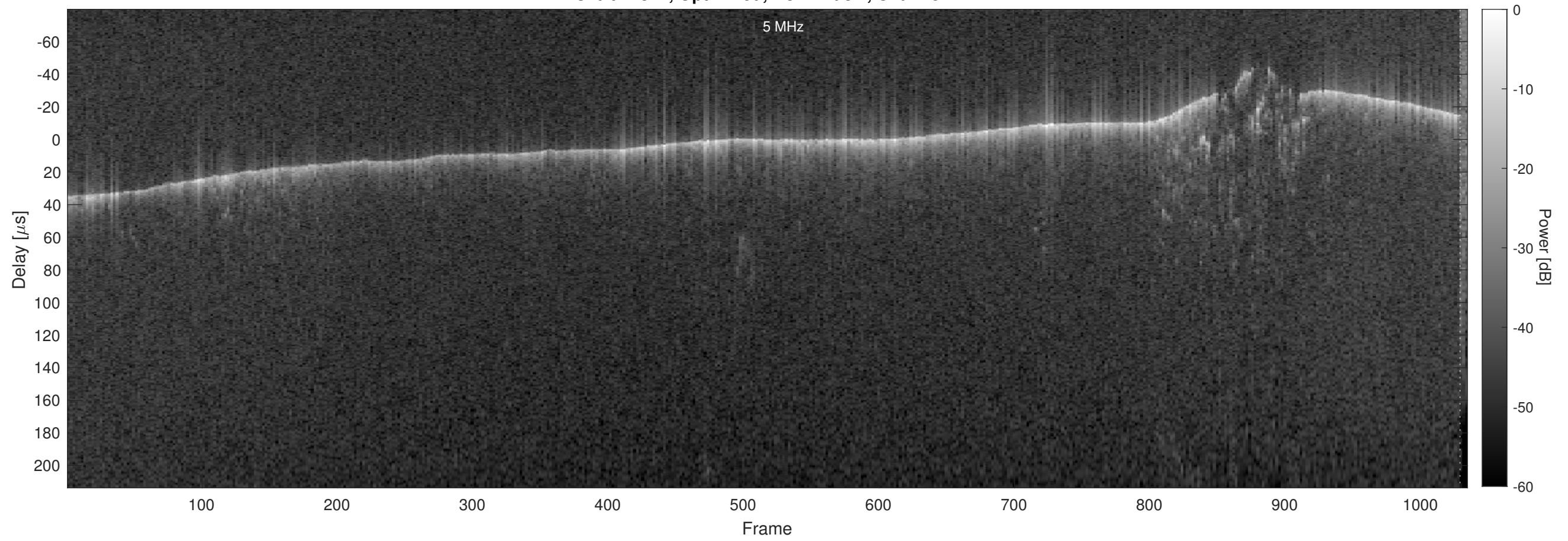
Orbit 17821, Optimized, No Window, Channel 2
