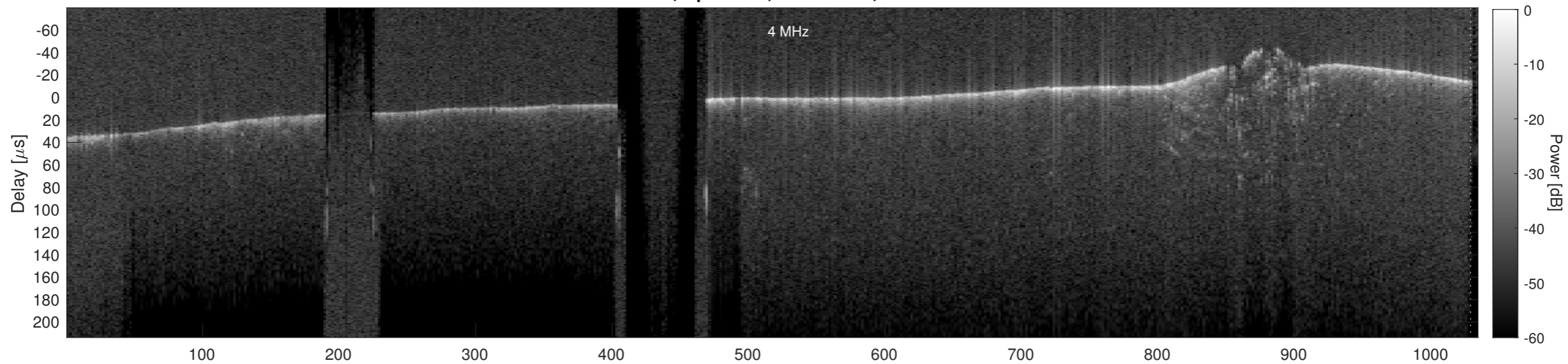
Orbit 17821, Cluttergram
