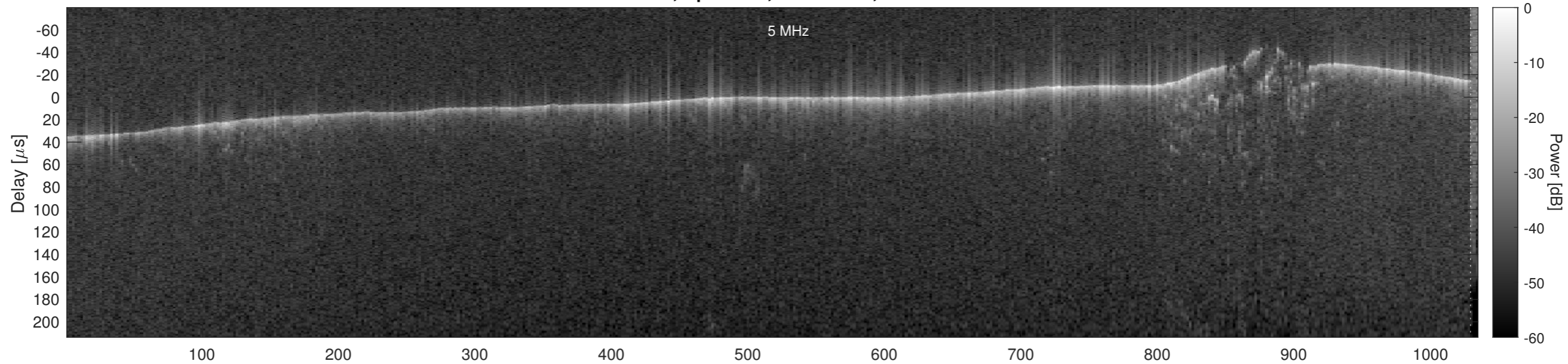
Orbit 17821, Optimized, No Window, Channel 2
