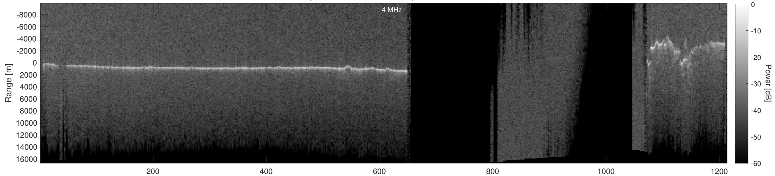
Orbit 17822, Depth-Corrected Cluttergram
