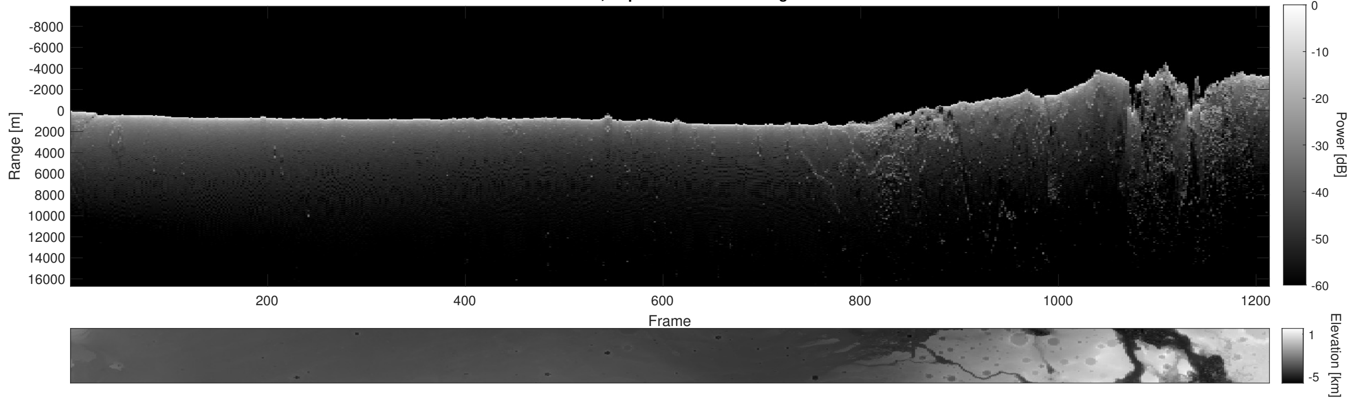
Orbit 17822, Depth-Corrected Cluttergram
