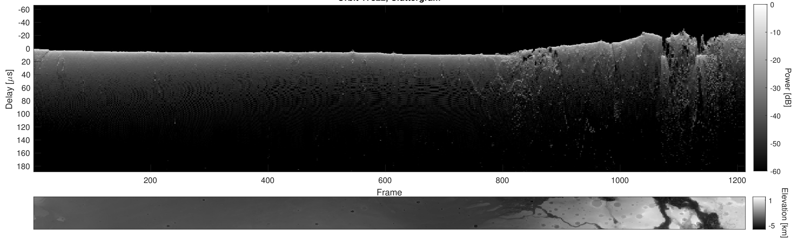
Orbit 17822, Cluttergram
