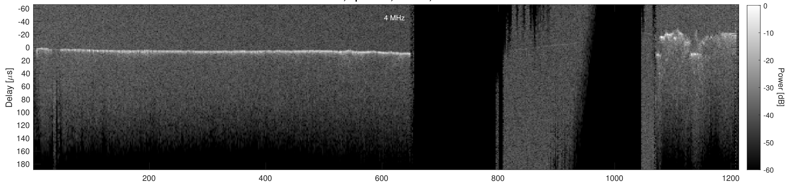
Orbit 17822, Cluttergram
