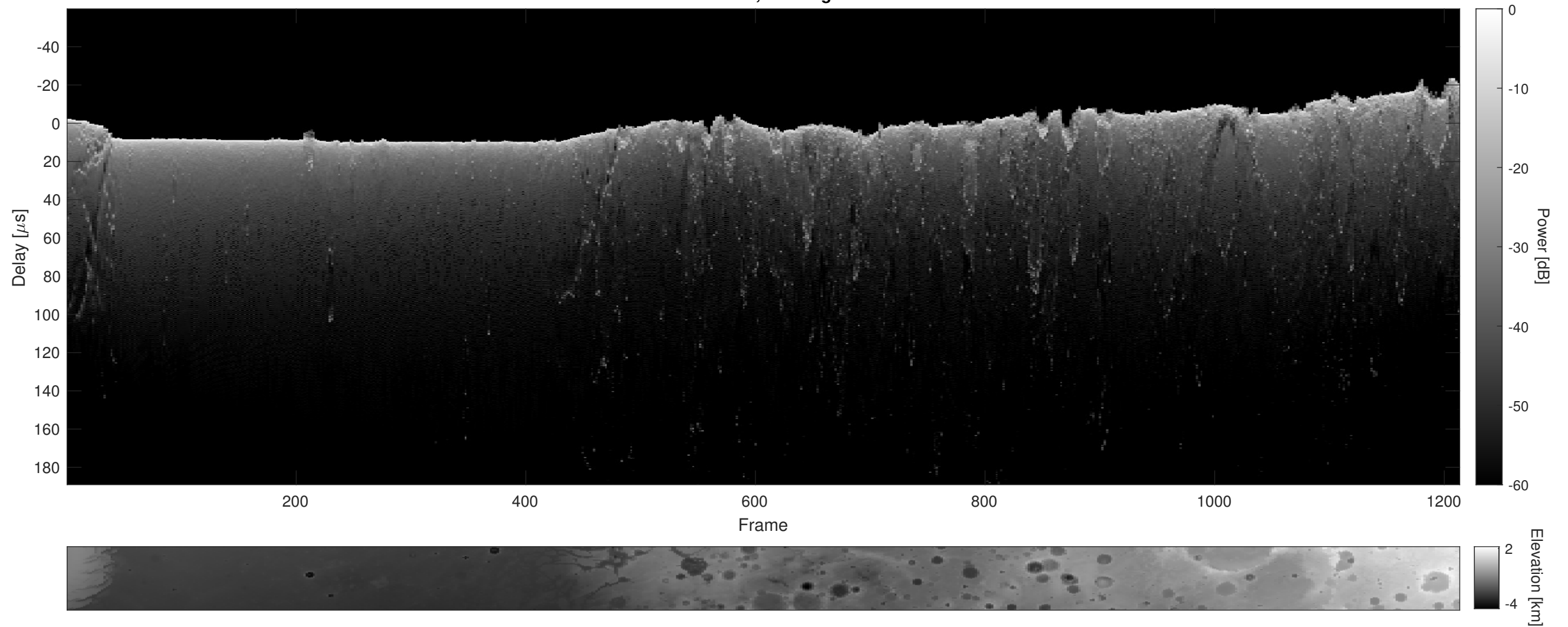
Orbit 17825, Cluttergram
