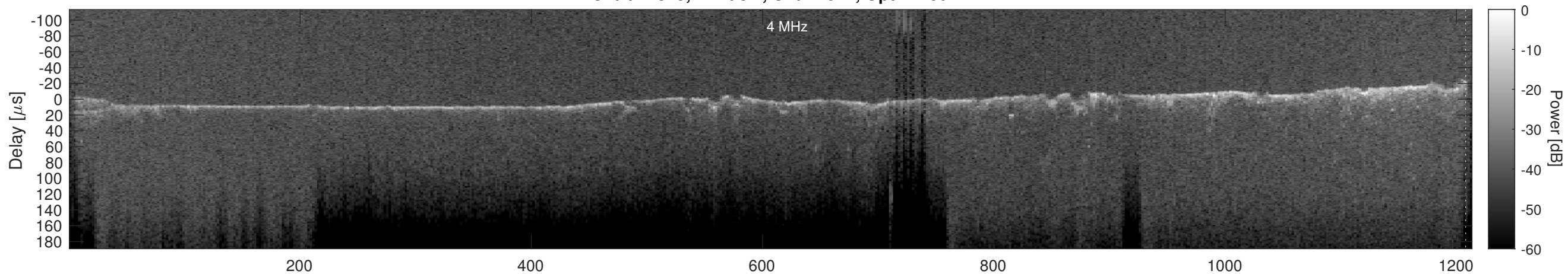
Orbit 17825, Cluttergram
