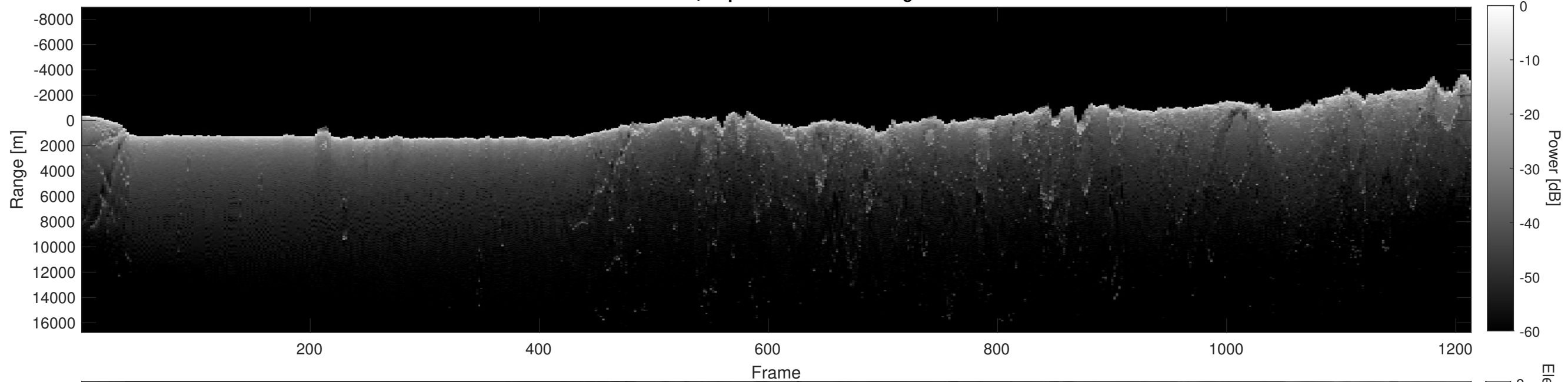
Orbit 17825, Depth-Corrected Cluttergram
