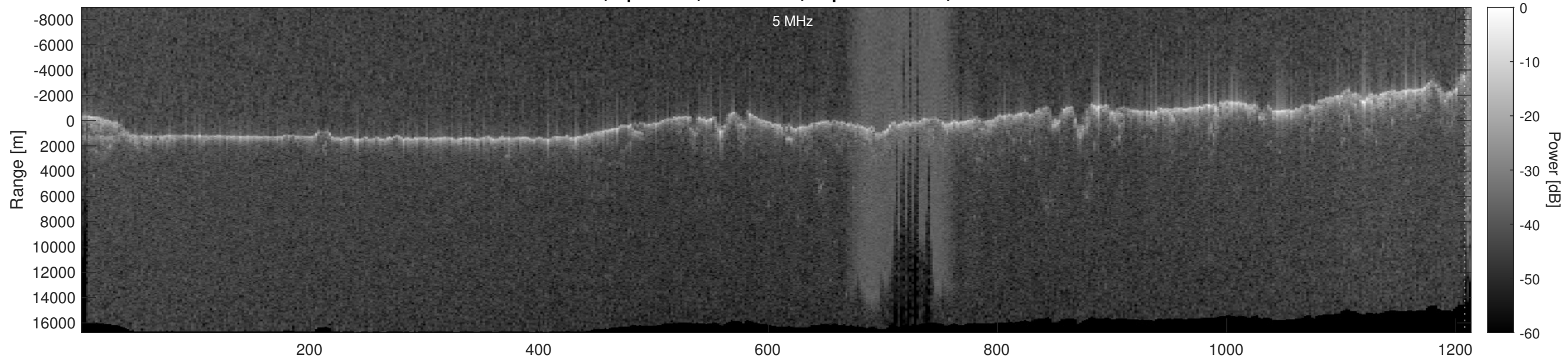
Orbit 17825, Optimized, No Window, Depth-Corrected, Channel 2
