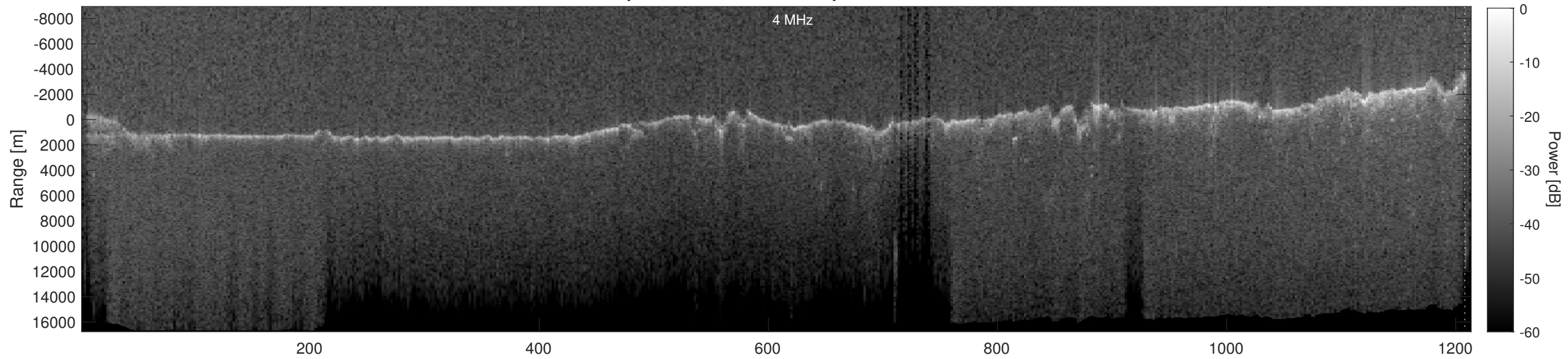
Orbit 17825, Depth-Corrected Cluttergram
