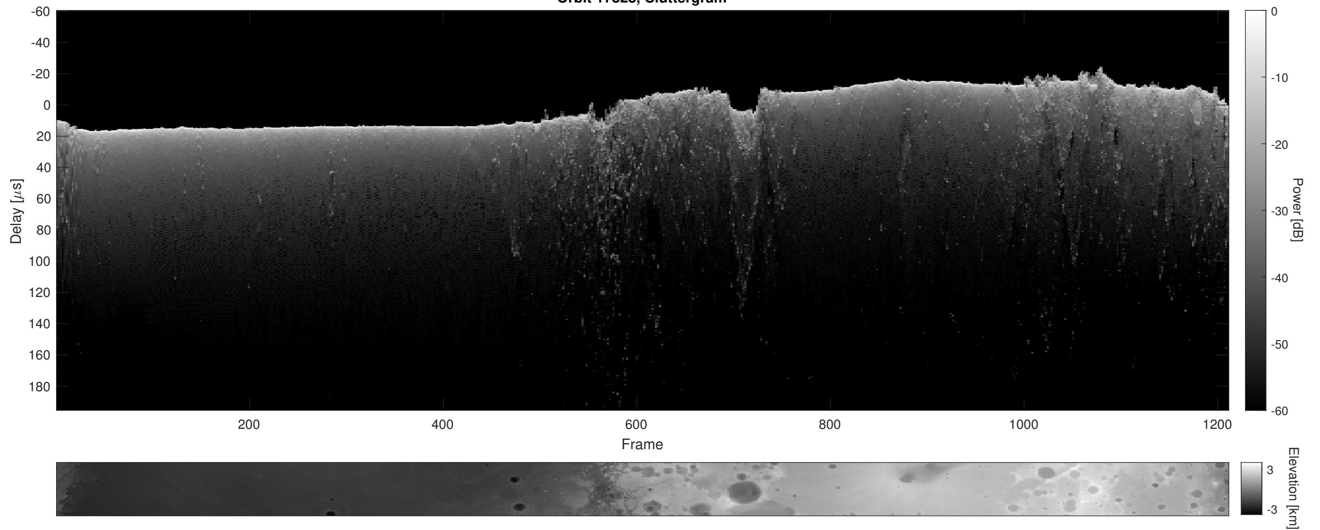
Orbit 17828, Cluttergram
