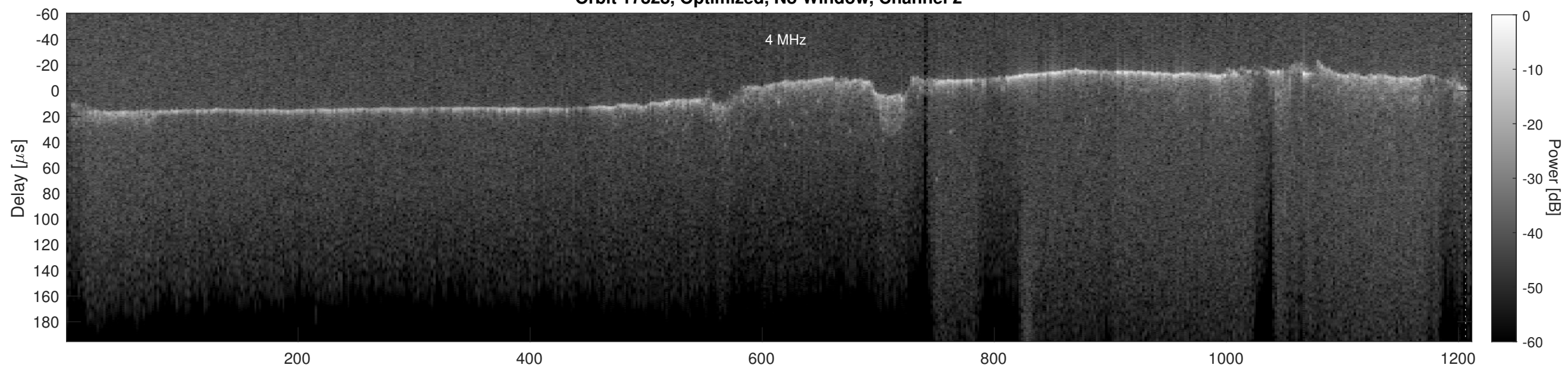
Orbit 17828, Cluttergram
