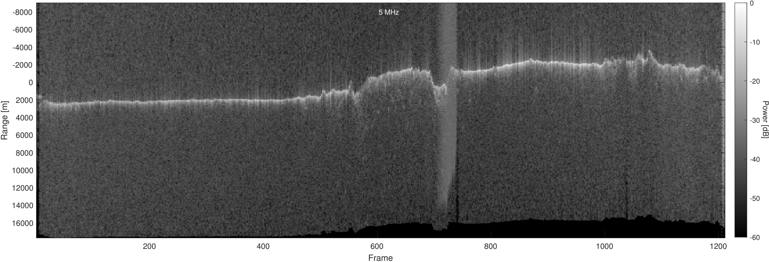
Orbit 17828, Optimized, No Window, Depth-Corrected, Channel 2
