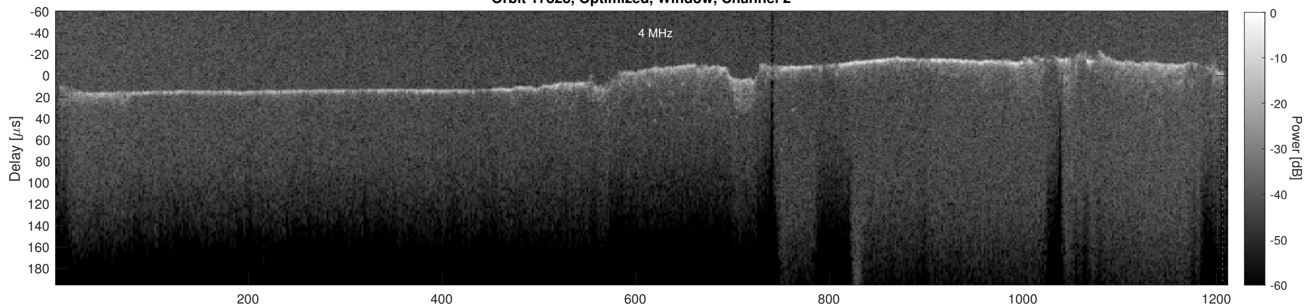
Orbit 17828, Cluttergram
