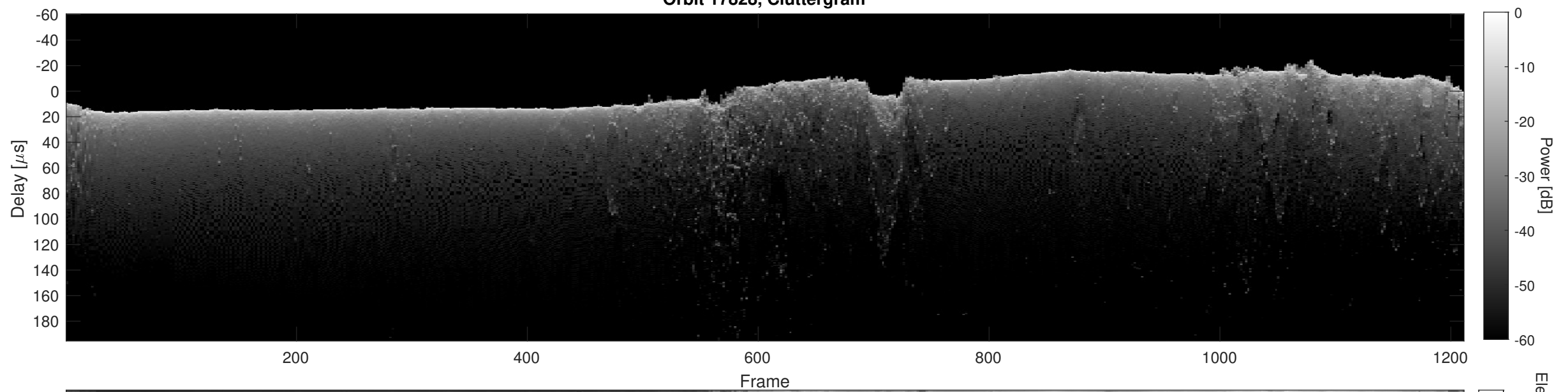
Orbit 17828, Cluttergram
