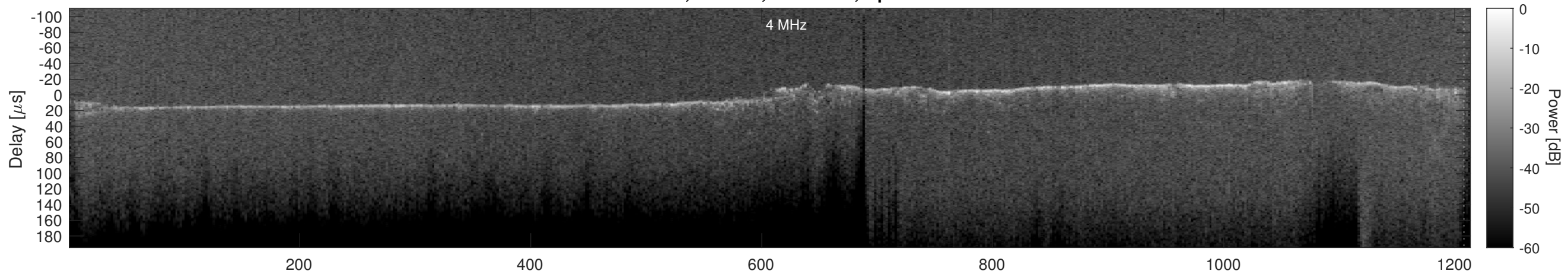
Orbit 17835, Cluttergram
