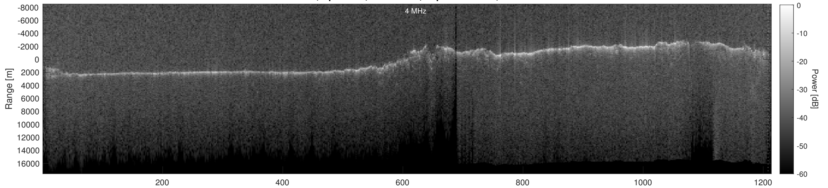
Orbit 17835, Depth-Corrected Cluttergram
