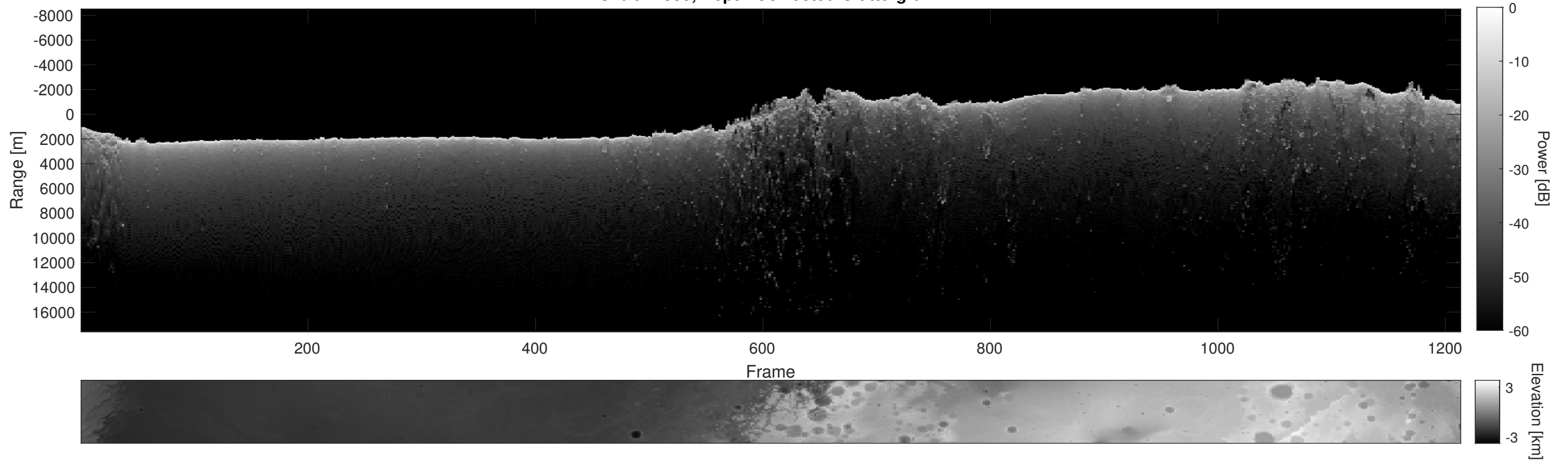
Orbit 17835, Depth-Corrected Cluttergram
