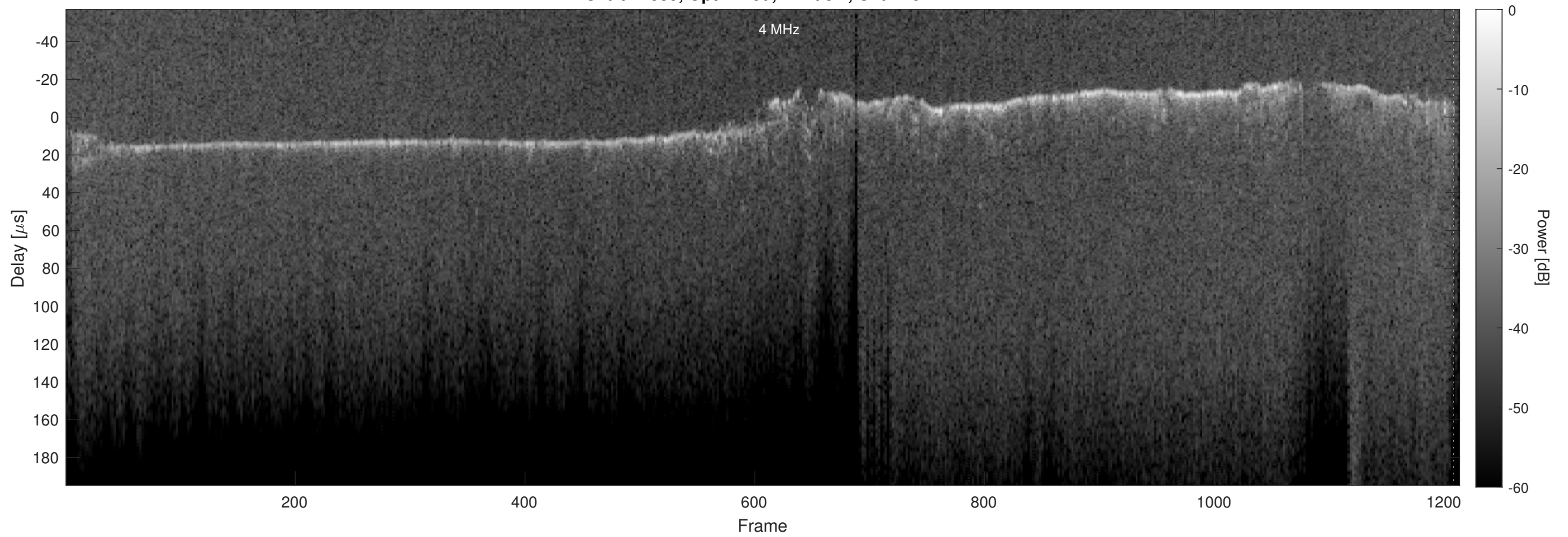
Orbit 17835, Optimized, Window, Channel 2
