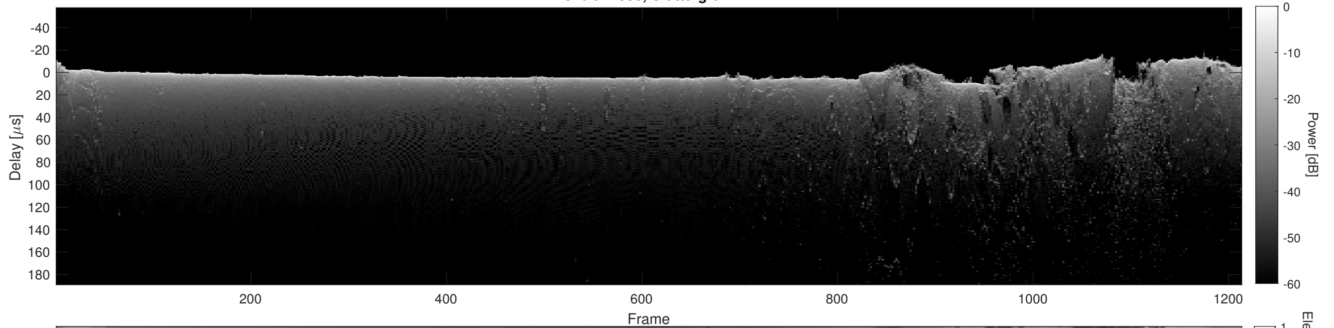
Orbit 17836, Cluttergram
