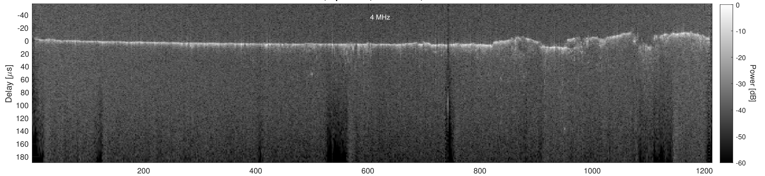
Orbit 17836, Cluttergram
