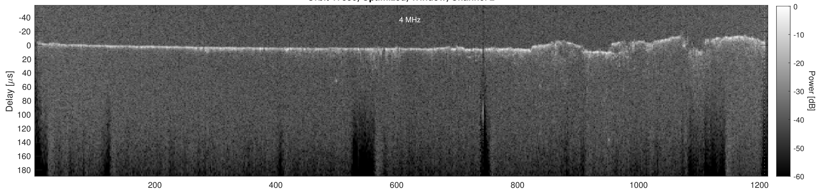
Orbit 17836, Cluttergram
