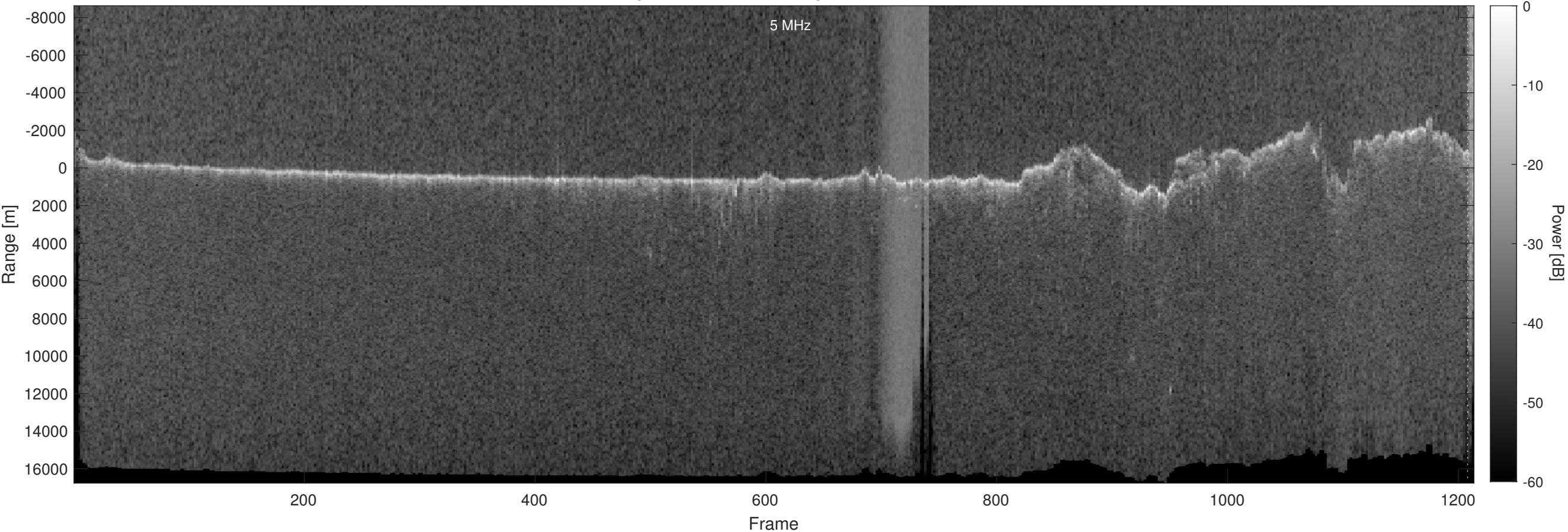
Orbit 17836, Optimized, Window, Depth-Corrected, Channel 2
