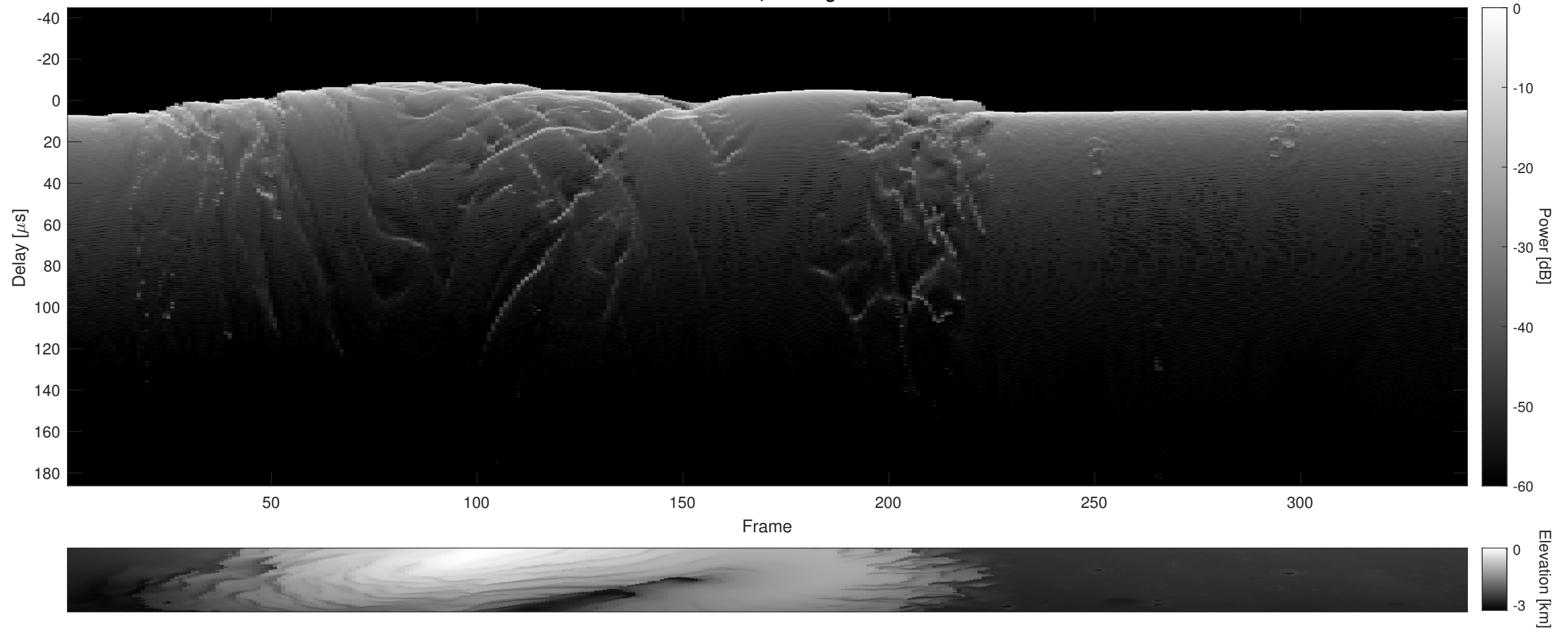
Orbit 17920, Cluttergram
