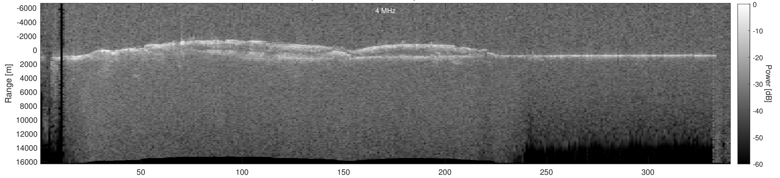
Orbit 17920, Depth-Corrected Cluttergram
