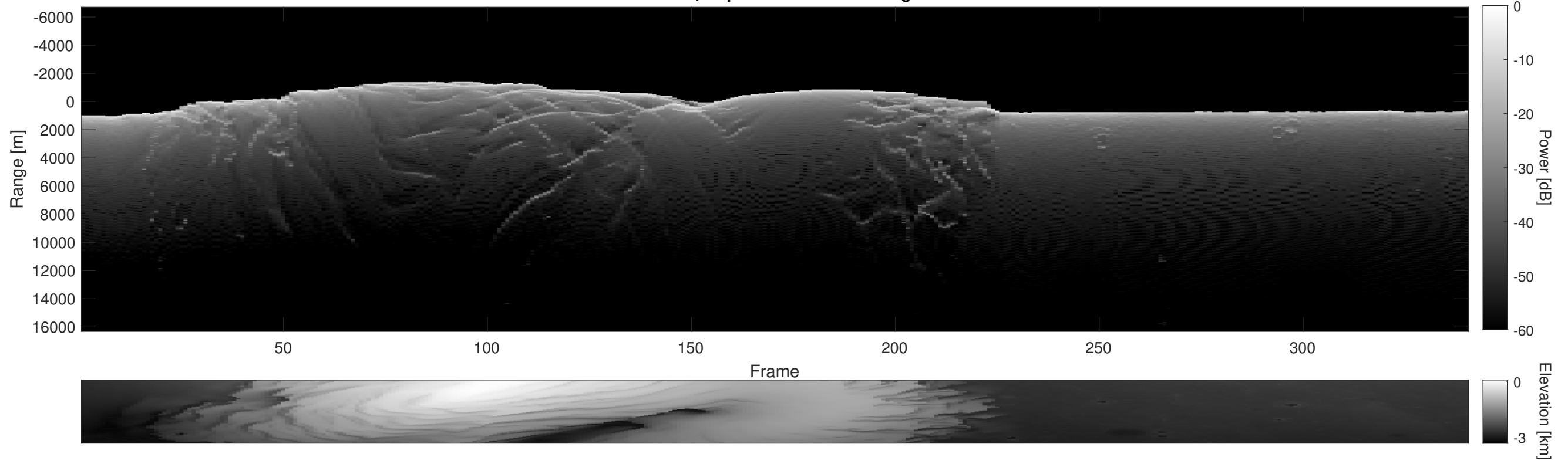
Orbit 17920, Depth-Corrected Cluttergram
