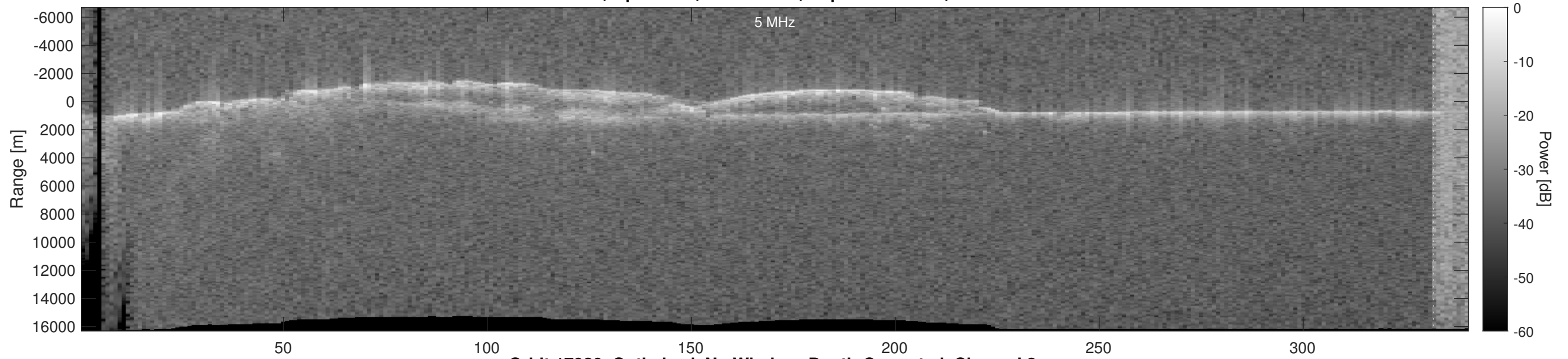
Orbit 17920, Optimized, No Window, Depth-Corrected, Channel 2
