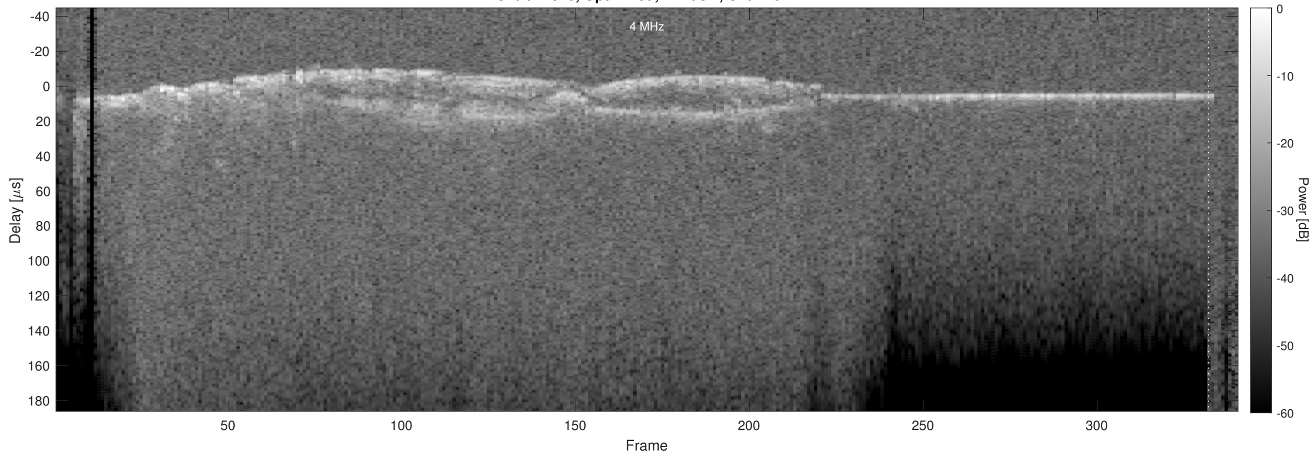
Orbit 17920, Optimized, Window, Channel 2
