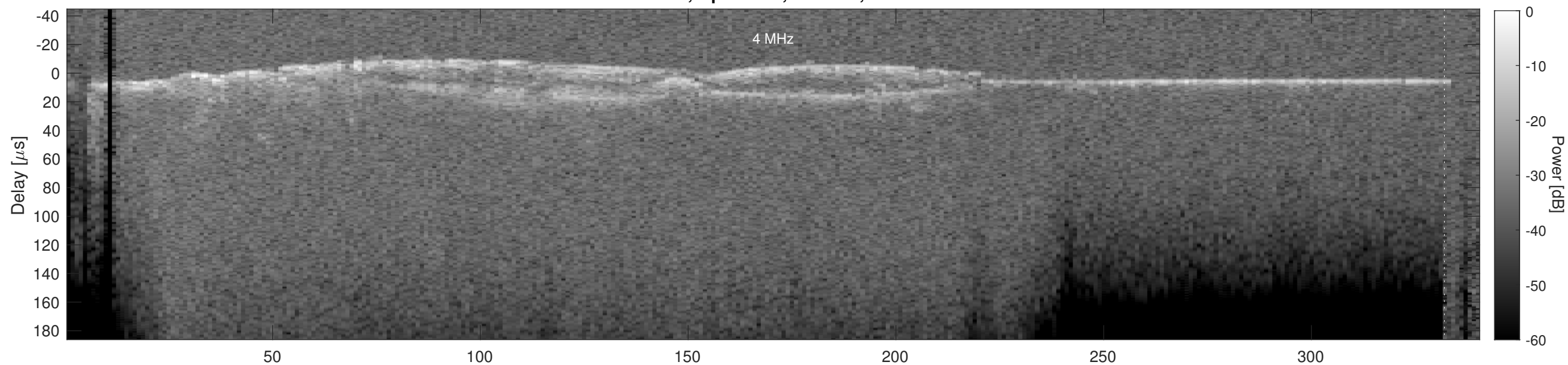
Orbit 17920, Cluttergram
