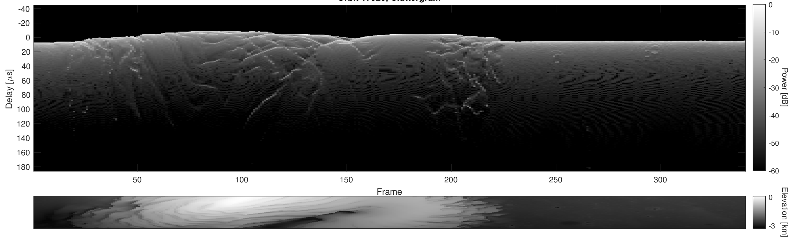
Orbit 17920, Cluttergram
