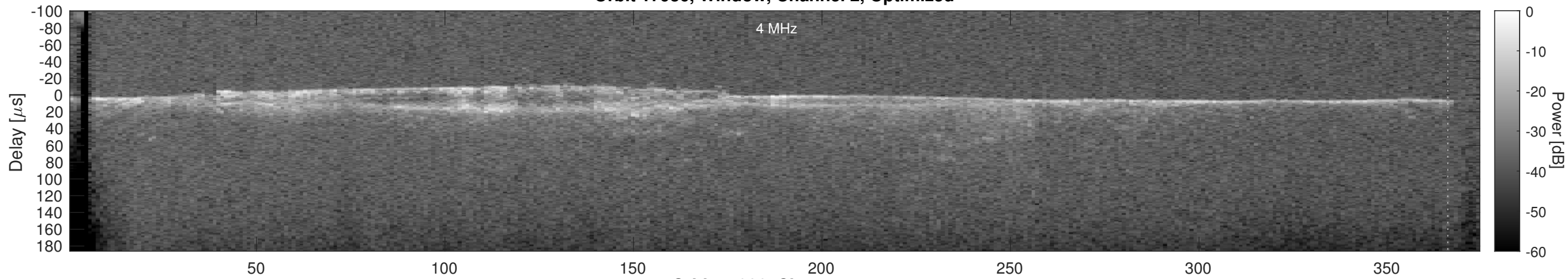
Orbit 17936, Cluttergram
