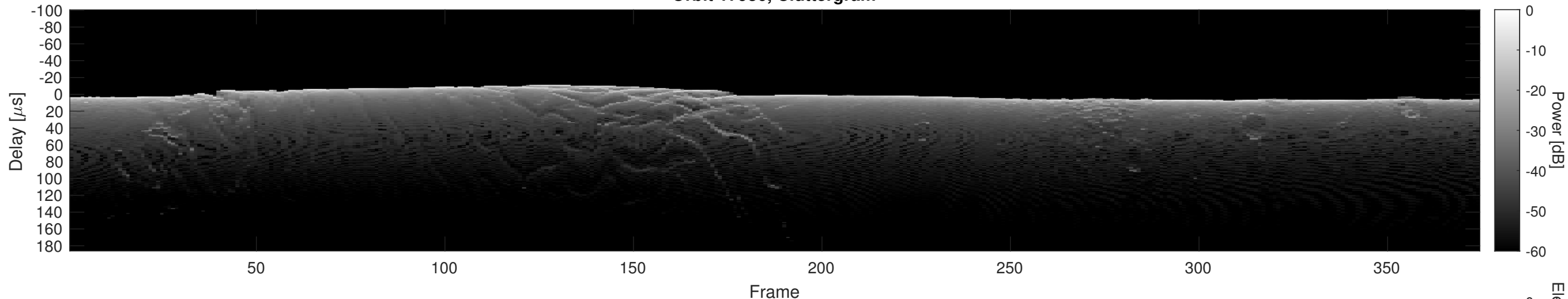
Orbit 17936, Cluttergram
