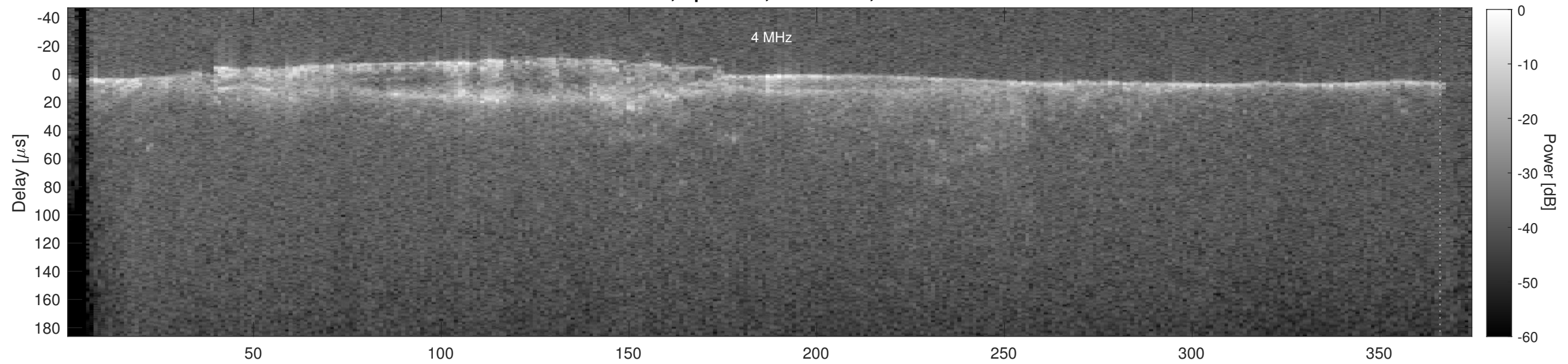
Orbit 17936, Cluttergram
