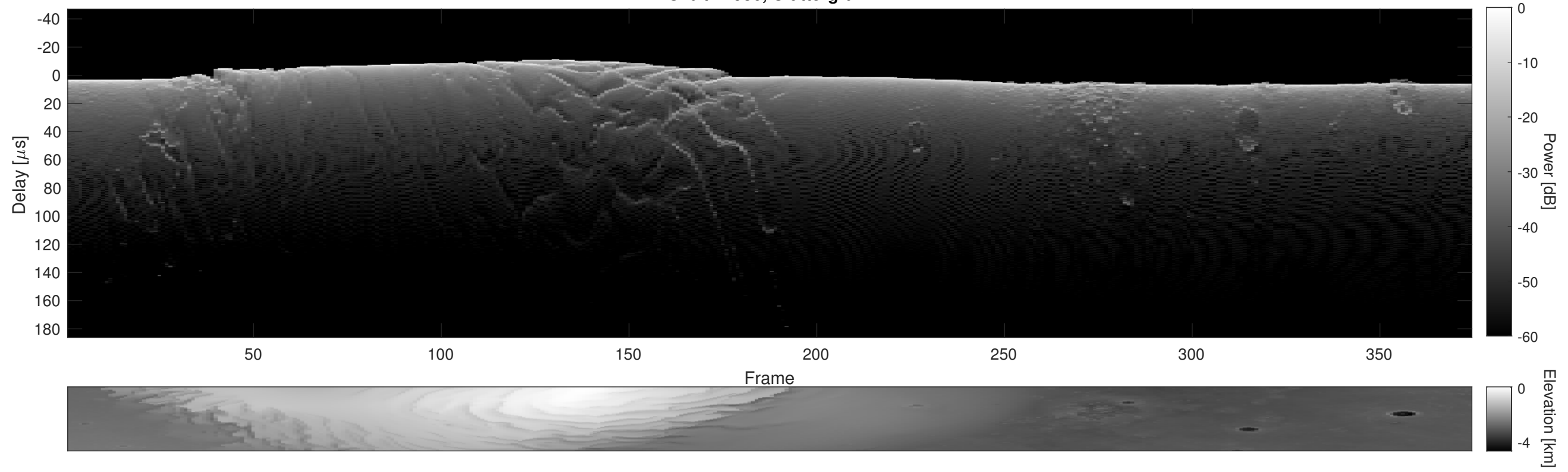
Orbit 17936, Cluttergram
