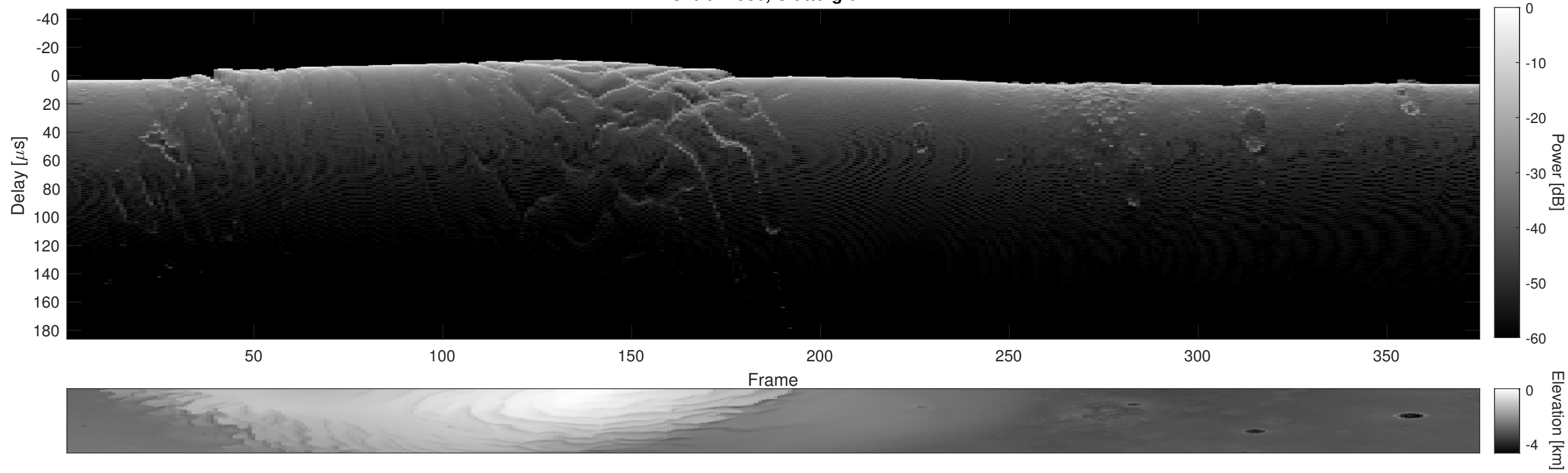
Orbit 17936, Cluttergram
