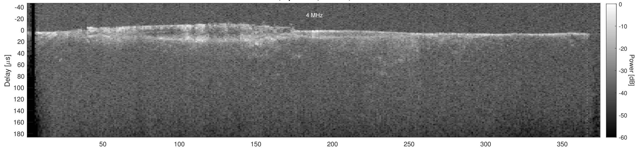
Orbit 17936, Cluttergram
