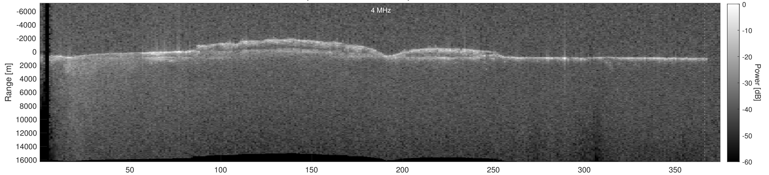
Orbit 17938, Depth-Corrected Cluttergram
