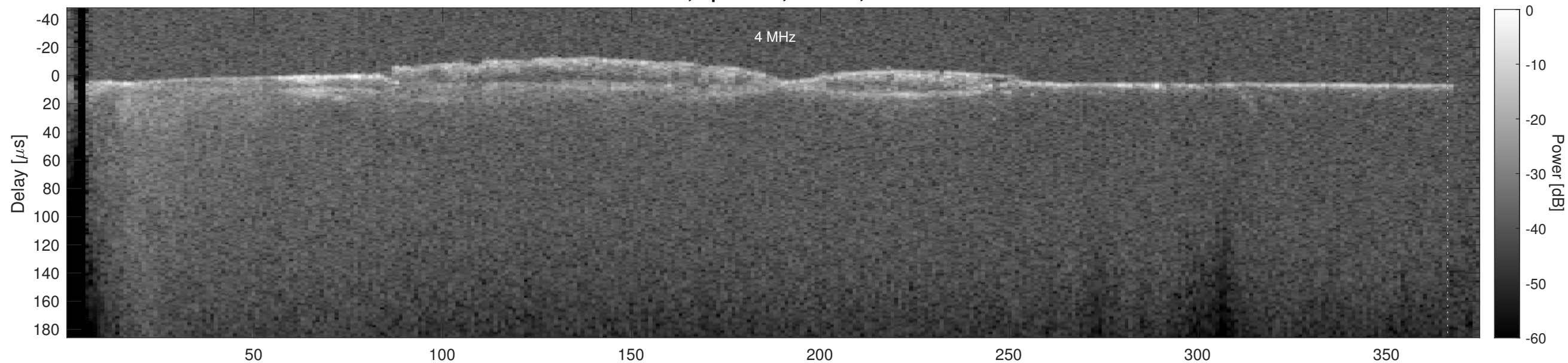
Orbit 17938, Cluttergram
