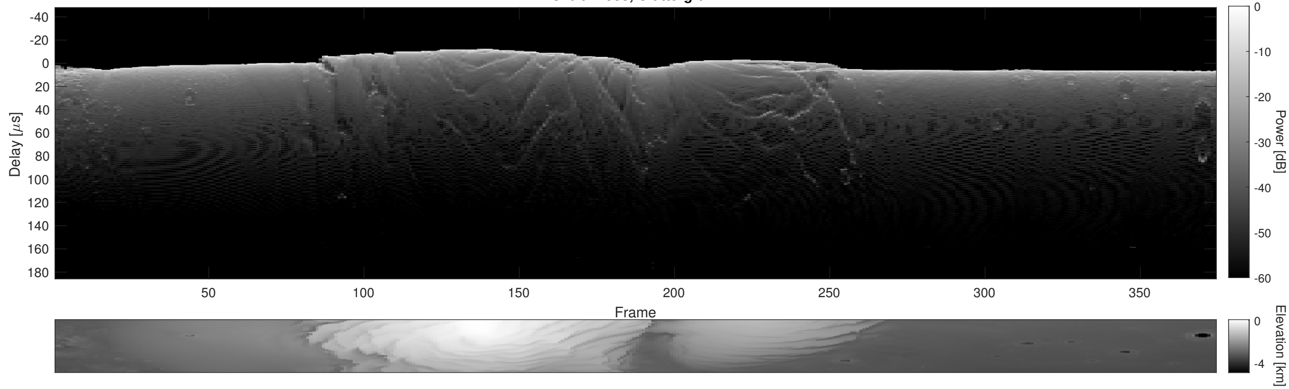
Orbit 17938, Cluttergram
