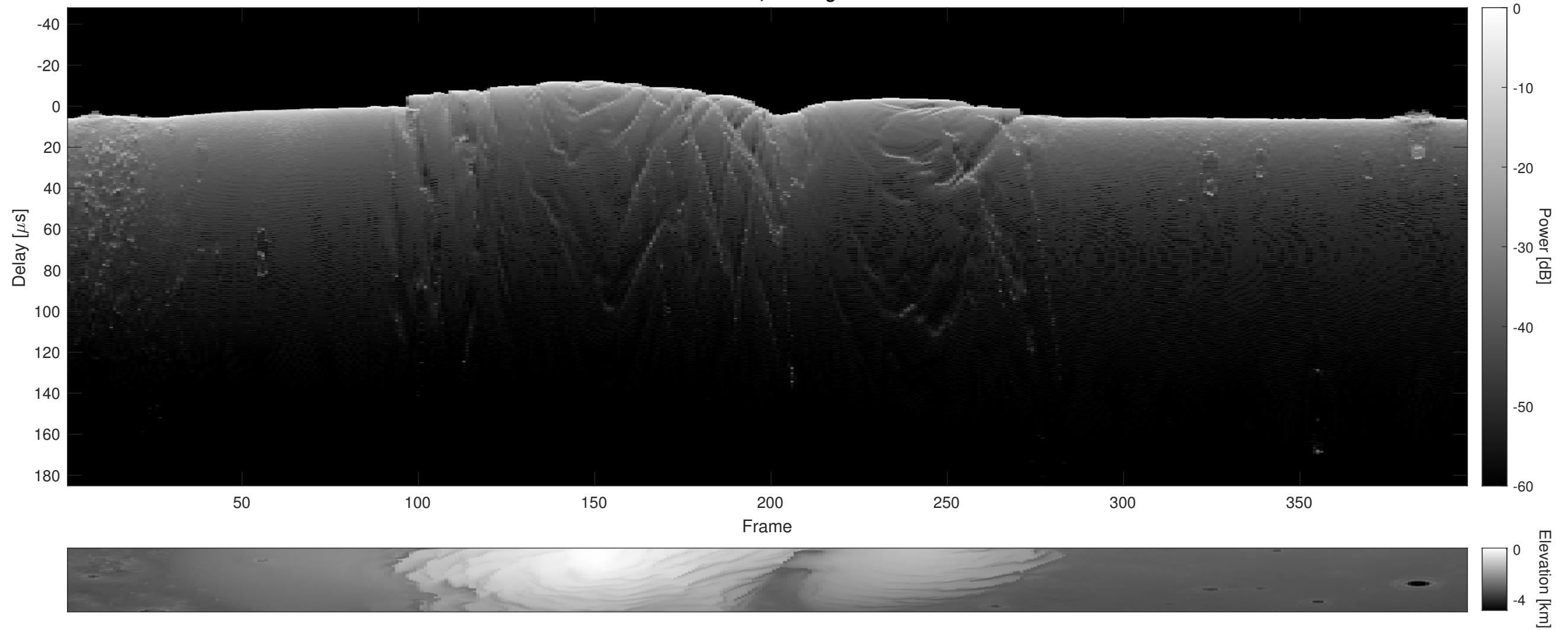
Orbit 17945, Cluttergram
