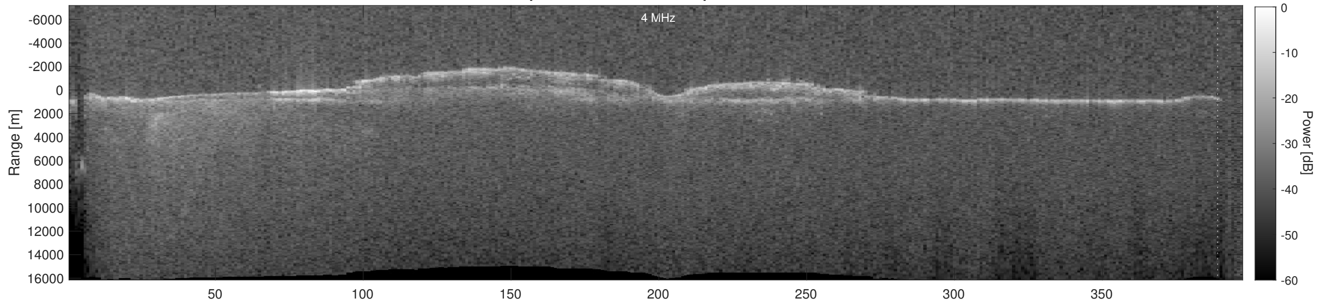
Orbit 17945, Depth-Corrected Cluttergram
