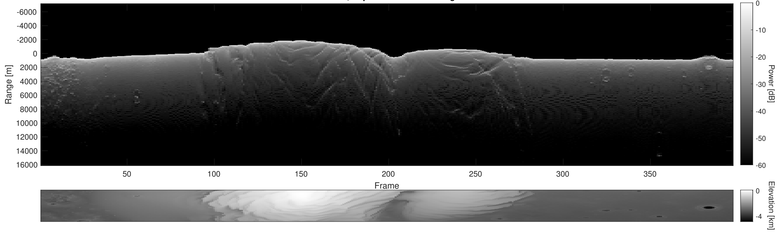
Orbit 17945, Depth-Corrected Cluttergram
