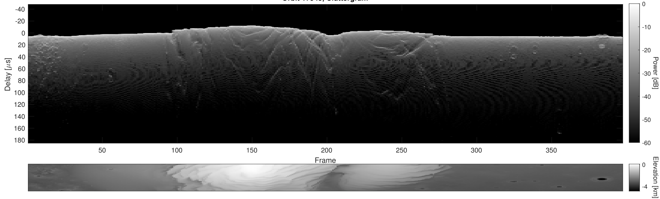
Orbit 17945, Cluttergram
