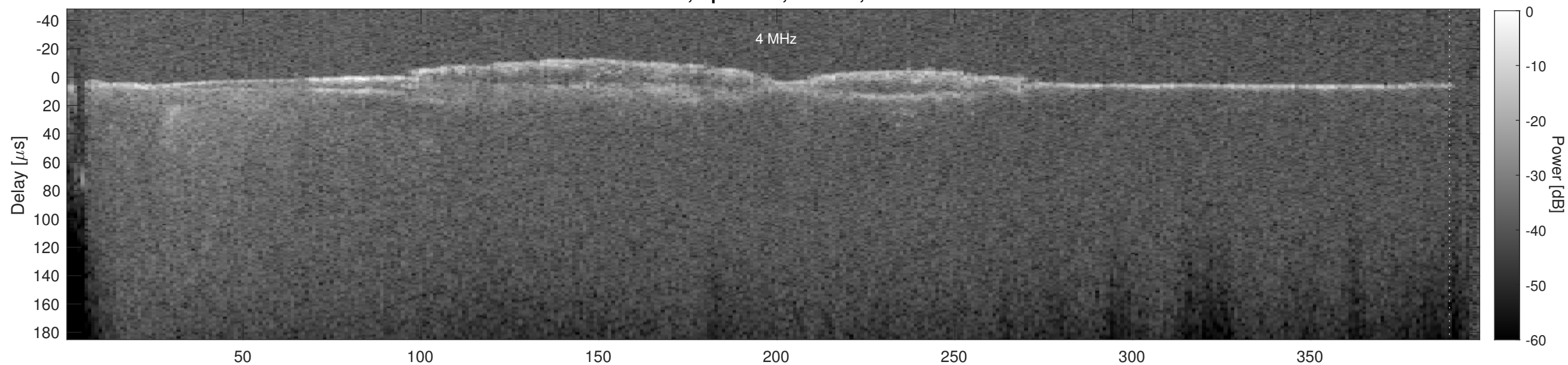
Orbit 17945, Cluttergram
