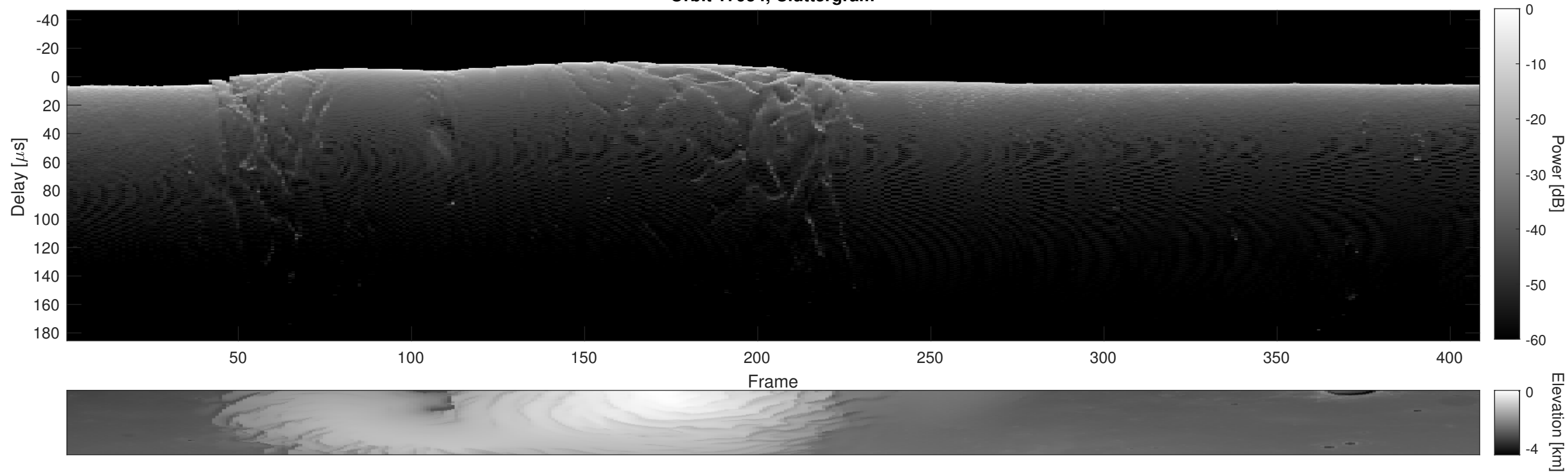
Orbit 17954, Cluttergram
