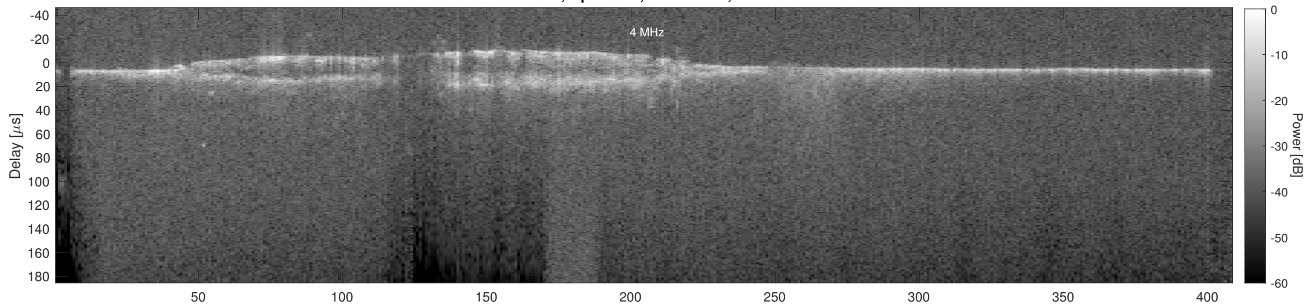
Orbit 17954, Cluttergram
