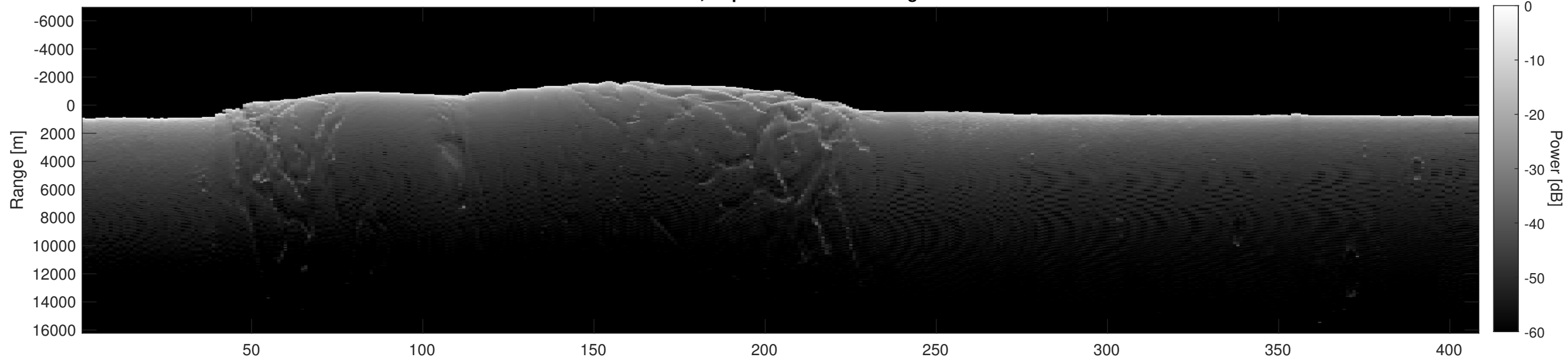
Orbit 17954, Depth-Corrected Cluttergram
