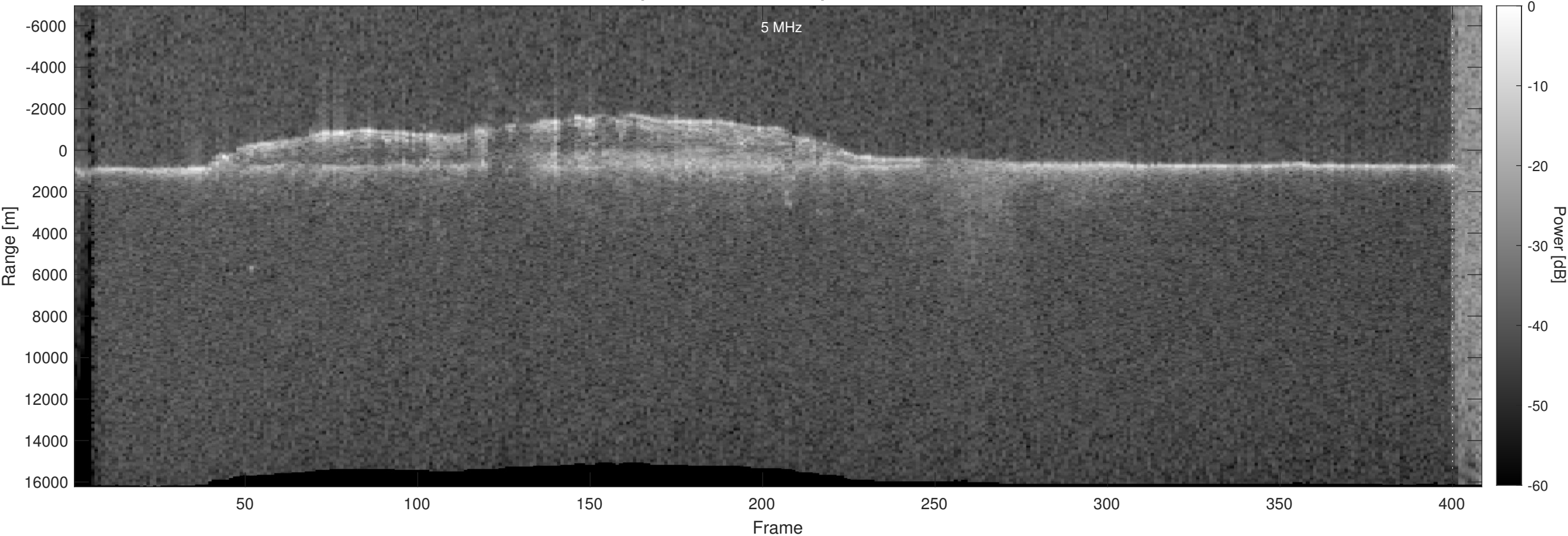
Orbit 17954, Optimized, Window, Depth-Corrected, Channel 2
